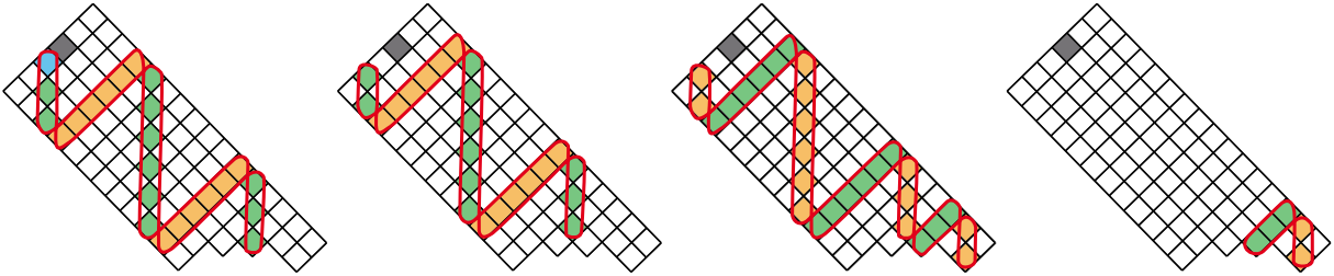
FIGURE 2.10. Proof of Lemma 2.3: an external cell c and its image under h(D)^{-2} . On the left, h(D)^{-1}(\gamma(c)) is a curve that turns positively around blocks of orange cells and negatively around blocks of green (and blue) cells. On the center left, the image under h(D)^{-1} of the curve h(D)^{-1}(\gamma(c)) , except the part that winds around the blue cell. On the center right, the image under h(D)^{-1} of the part of the curve h(D)^{-1}(\gamma(c)) that winds around the blue cell. On the right, the concatenation of those two parts is the curve h(D)^{-2}(\gamma(c)) , it is a curve that only winds around some cells of the mixing zone of D .
