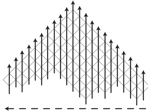
FIGURE 2.5. Decomposition of the monodromy h(D) as the product of the Dehn twists around the \chi(D) elementary curves on S(D) (that is, those curves that turns once around the cells of D ). The order is from right to left, and in every column from bottom to top.
