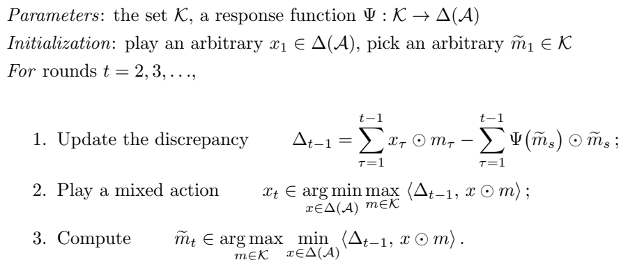
Figure 3: A generalization of the strategy of Bernstein and Shimkin (2015).
