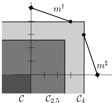
Figure 1: Graphical representation of m^\dagger and m^\sharp and of different expansions \mathcal{C}_\alpha .
