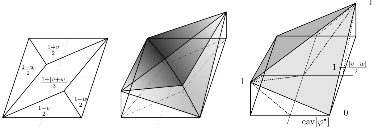
Figure 6: Representations in 2D – 3D of \varphi^{x^*} (left and center) and 3D representation of \text{cav}[\varphi^*] .
