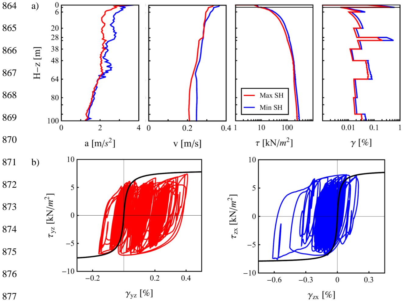
878 Figure 10. 1D-3C seismic response of soil profile MYGH09, during the 2011 Tohoku 879 earthquake, in both horizontal directions of motion: acceleration, velocity, strain and stress with 880 depth (a); shear stress-strain loops at 2 m depth (b).
