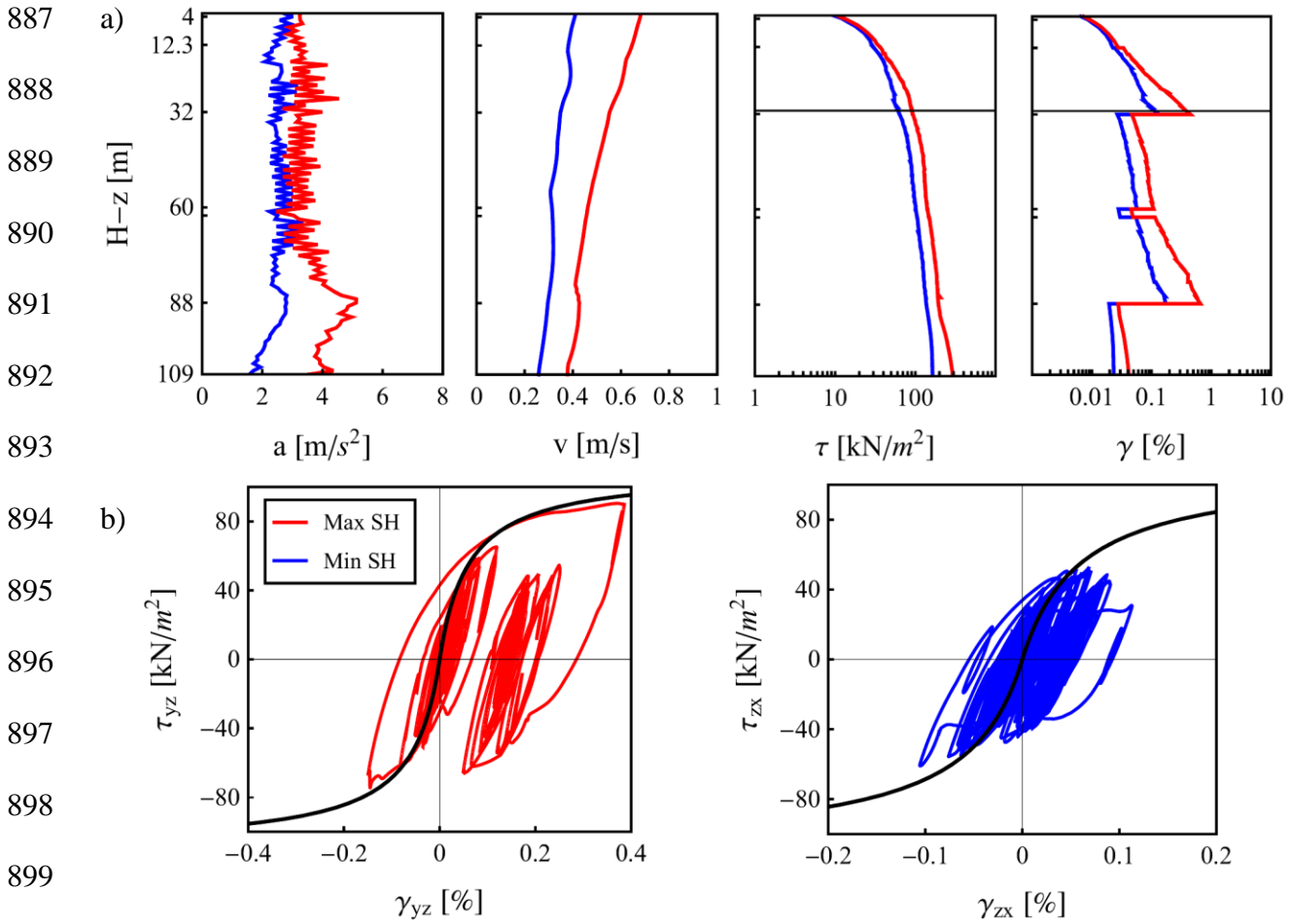
887 888 889 890 891 892 893 894 895 896 897 898 899 900 Figure 11. 1D-3C seismic response of soil profile FKSH20, during the 2011 Tohoku earthquake, 901 in both horizontal directions of motion: acceleration, velocity, strain and stress with depth (a); 902 shear stress-strain loops at 31 m depth (b).
