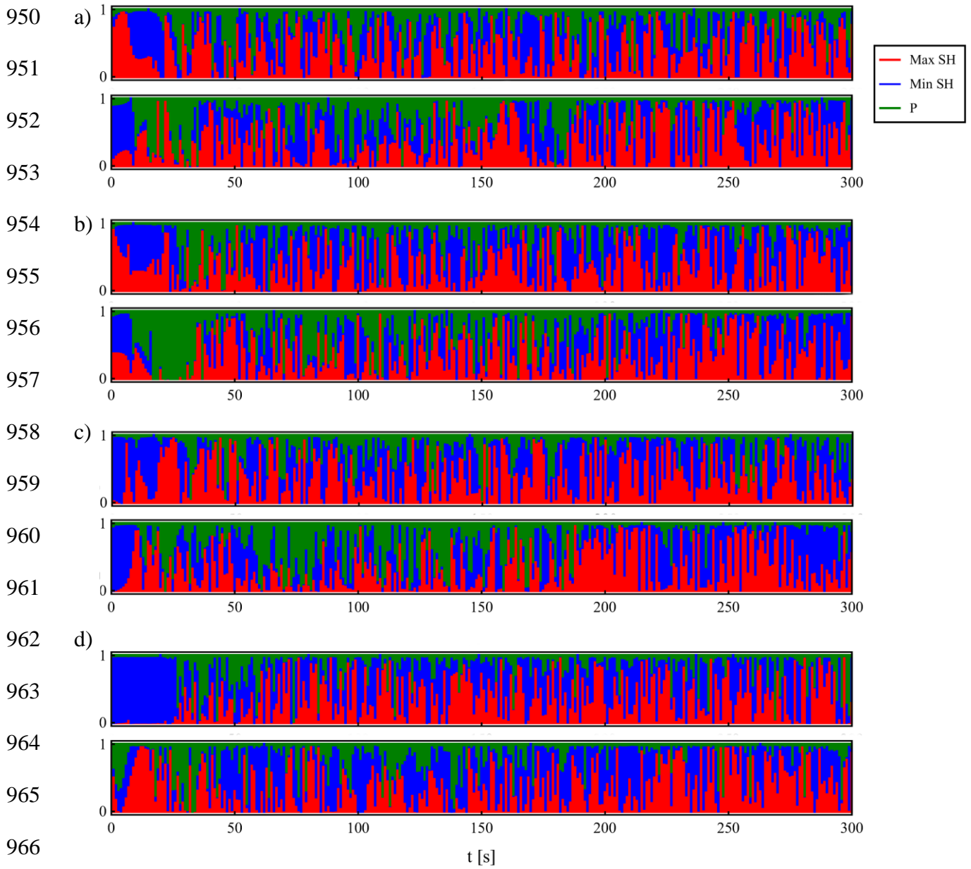
967 Figure 14. Recorded (top) and numerical (bottom) normalized polarization of seismic waves in 968 terms of acceleration at the surface of soil profiles MYGH09 (a), FKSH20 (b), IWTH04 (c) and 969 IBRH12 (d). Max SH is the PGA horizontal direction and P is the vertical direction.
