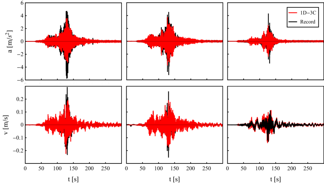
812 Figure 7. Time history of measured and numerical acceleration (top) and velocity (bottom), in 813 directions NS (left), EW (middle) and UD (right), at the surface of soil profile IBRH12, during 814 the 2011 Tohoku earthquake.
