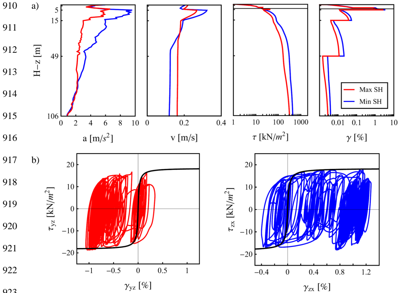
924 Figure 12. 1D-3C seismic response of soil profile IWTH04, during the 2011 Tohoku earthquake, 925 in both horizontal directions of motion: acceleration, velocity, strain and stress with depth (a); 926 shear stress-strain loops at 4 m depth (b).
