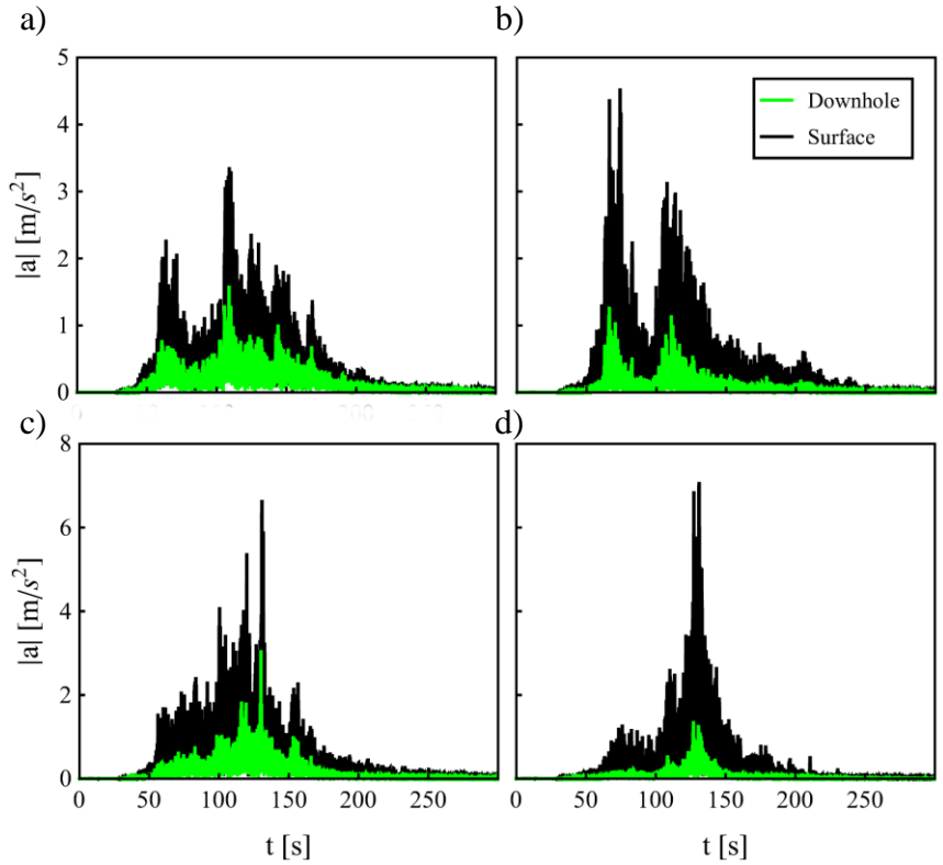
Figure 3. Time history of measured acceleration modulus at the base and surface of soil profiles MYGH09 (a), IWTH04 (b), FKSH20 (c) and IBRH12 (d), during the 2011 Tohoku earthquake.
