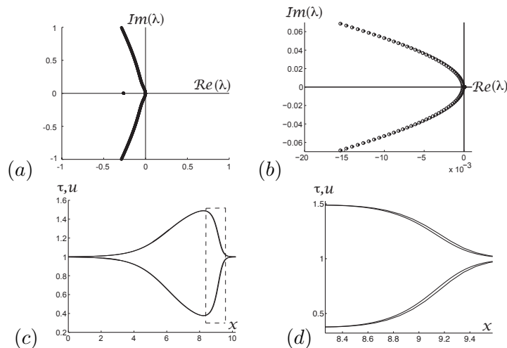
Figure 10: In Figure (a), we have superimposed the spectrum of an exact periodic traveling wave solution of (2.2) and the spectrum associated to a periodically extended version of the homoclinic profile found in Section 5.2.2 with the same period. As one can see, the spectra are nearly identical: in Figure (b) we zoom in on Figure (a) near the origin, showing the very slight discrepancy between the spectrum of the exact periodic (circles) and the periodically extended homoclinic (solid dots). Again, this spectrum was found using SpectrUW. Continuing, in Figure (c) we superimpose the profiles of the exact periodic traveling wave solution (bold) with the periodically extended homoclinic (thin) with the same period. Again, these profiles are nearly identical: in Figure (d) we zoom in on the dashed box in Figure (c) to illustrate the close agreement of these profiles.
