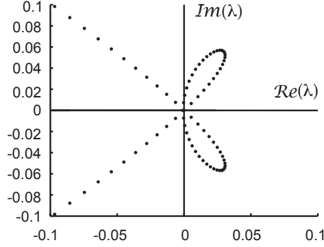
Figure 1: Here, we depict a numerical sampling of the (continuous) essential spectrum of the PDE (2.6), plotted as \Re(\lambda) vs. \Im(\lambda) , when linearized about a constant state, for values of the parameters at which the constant state undergoes a Hopf bifurcation when considered as a fixed point of the ODE (2.4). In this example, we have taken r = 2 , s = 4 , u_0 = 0.96 , q = u_0 + c/u_0^2 , \nu = 0.1 , F = 6 , and c = c_s = 0.57052639 (corresponding to the Hopf bifurcation). Notice the triple degeneracy of the \lambda = 0 eigenvalue in this case.
