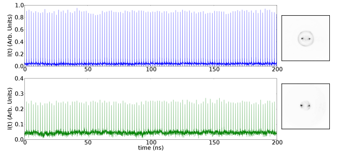
Figure 5: VCSEL time traces emission and corresponding far-field emission profile in the mode-locking regime for two values of the VCSEL bias. Upper panel J = 703\text{mA} , Lower Panel J = 285\text{mA}
