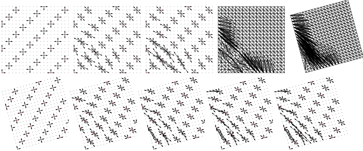
Figure 5: Top: Algorithm 2, for the classical monopolist problem (1) on [1, 2]^2 with a 20 \times 20 grid, converges in 2 stencil refinement steps (using the extended candidates \hat{\mathcal{V}}_\rho , \rho := 1.5 ). Bottom: 4 refinement steps are needed with a different density of customers, uniform on the square [1, 2]^2 rotated by \pi/12 . Top right: u -Delaunay triangulations associated with the respective discrete solutions, for illustration of Theorem 1.13.
