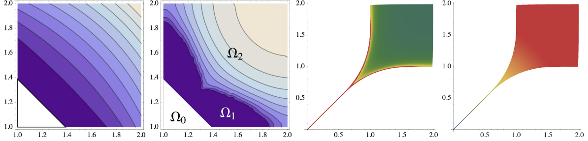
Figure 1: Numerical approximation U of the solution of the classical Monopolist’s problem (1), computed on a 50 \times 50 grid. Left: level sets of U , with U = 0 in white. Center left: level sets of \det(\text{Hessian } U) (with again U = 0 in white); note the degenerate region \Omega_1 where \det(\text{Hessian } U) = 0 . Center right: distribution of products sold by the monopolist. Right: profit margin of the monopolist for each type of product (margins are low on the one dimensional part of the product line, at the bottom left). Color scales on Figure 11.
