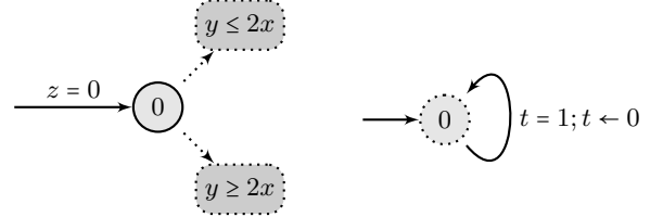
Figure 13: Accepting state q_f
