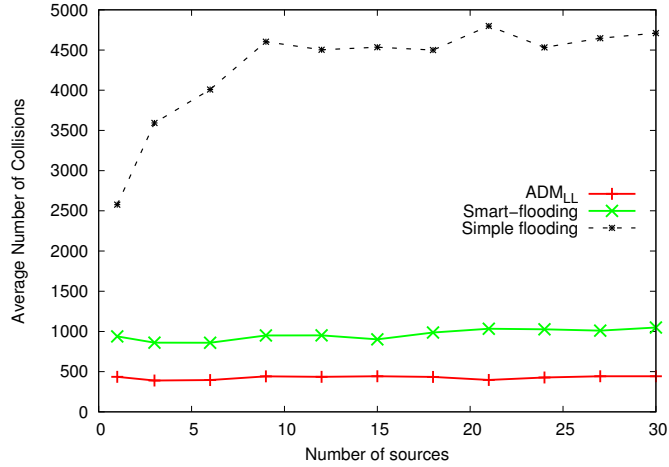
Figure 12: Collisions
