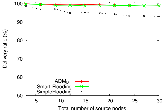
Figure 6: Delivery ratio
