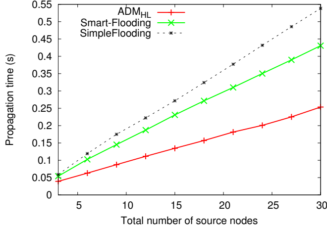
Figure 5: Propagation time
