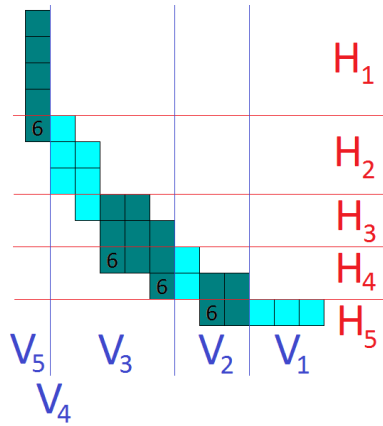
FIGURE 19. 6-boundary \partial^6(\lambda) = s^1(f) of the irreducible 6-shape \lambda = \varphi(f) .
