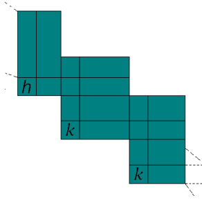
FIGURE 15. Partial k -shape s .
