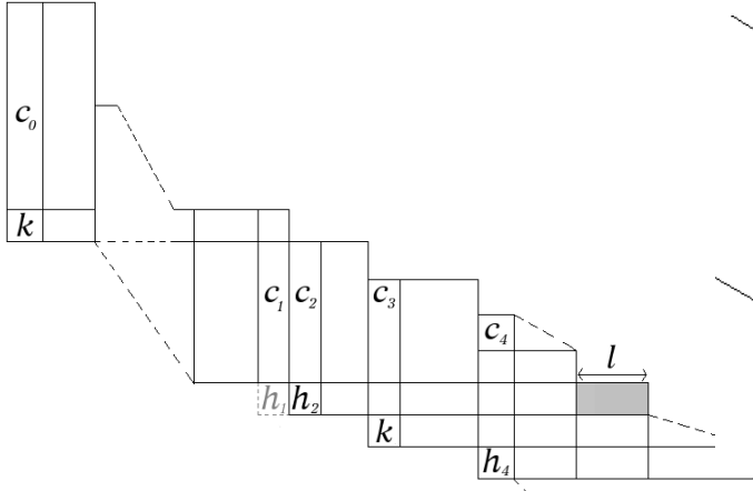
FIGURE 26. s^1(f)
