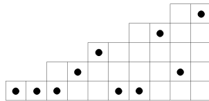
FIGURE 17. Surjective pistol f = (2, 8, 4, 10, 10, 6, 8, 10, 10, 10) \in SP_5 .
