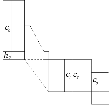
FIGURE 14. Between s and s \oplus_{t(j)}^k [(j+1)/2]^z .
