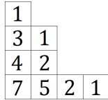
FIGURE 3. Ferrers diagram of the partition \lambda = (4, 2, 2, 1) .
