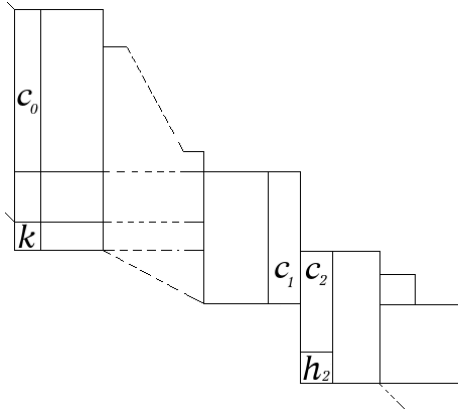
FIGURE 13. Partial k -shape s .
