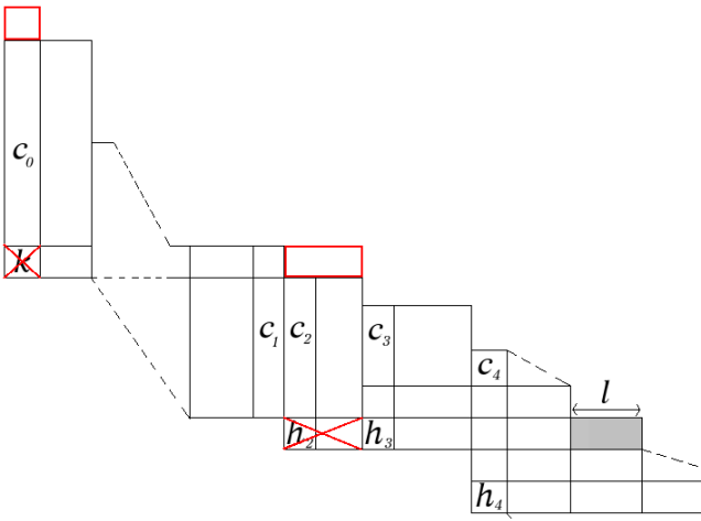
FIGURE 24. Between s^{j+1}(f) and s^j(f) .
