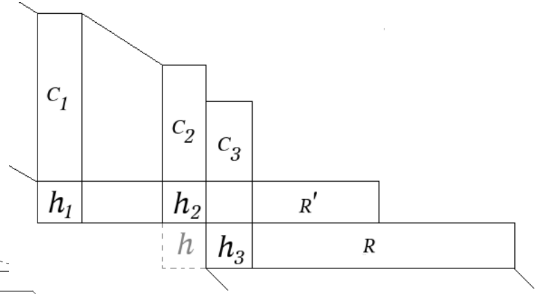
FIGURE 27. s^1
