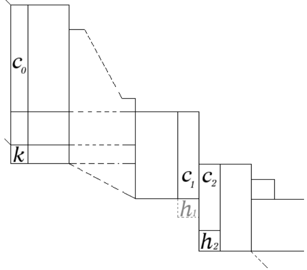
FIGURE 23. s^{j+1}(f) .
