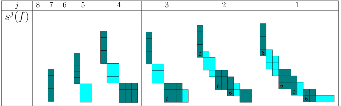
FIGURE 18. Sequence (s^j(f))_{j \in [8]} .
