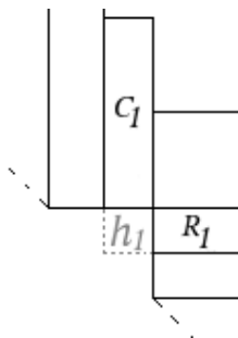
FIGURE 20. Anticoin labeled by its hook length h_1 .
