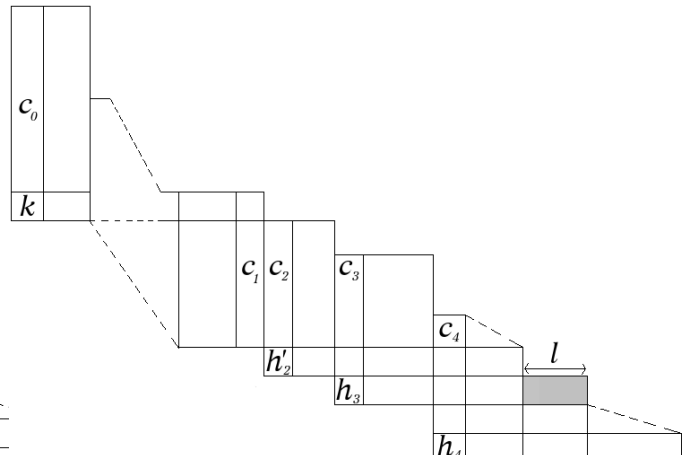
FIGURE 25. s^j(f) .
