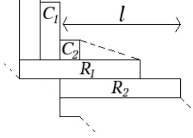
FIGURE 12. Partial k -shape s .
