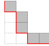
FIGURE 4. Skew partition \lambda \setminus \mu .
