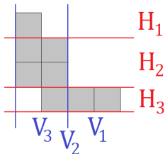
FIGURE 5. Skew partition \partial^5(\lambda) with \lambda = (4, 2, 2, 1) .
