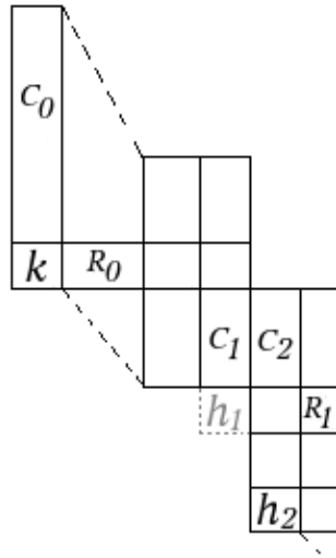
FIGURE 22. s^1(f) .
