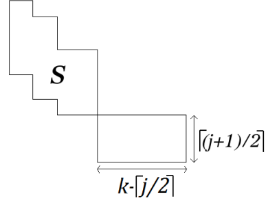
FIGURE 16. Partial k -shape s^{k-\lceil j/2 \rceil} .
