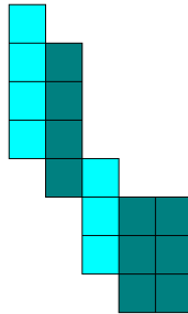
FIGURE 7. Partial 6-shape s \oplus_1 3^2 .
