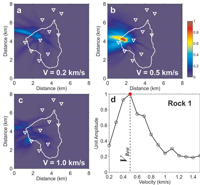
Figure 5. Location of mass wasting events in the Illgraben. (a–c) Probability density map (unit amplitude) for rock 1 location in the [29–29.5] Hz frequency band. Migration velocities are 0.2 (a), 0.5 (b) and 1.0 km s -1 (c). (d) Migration velocity analysis where the maximum amplitude corresponds to the best fit propagation velocity (0.5 km s -1 for rock 1).
