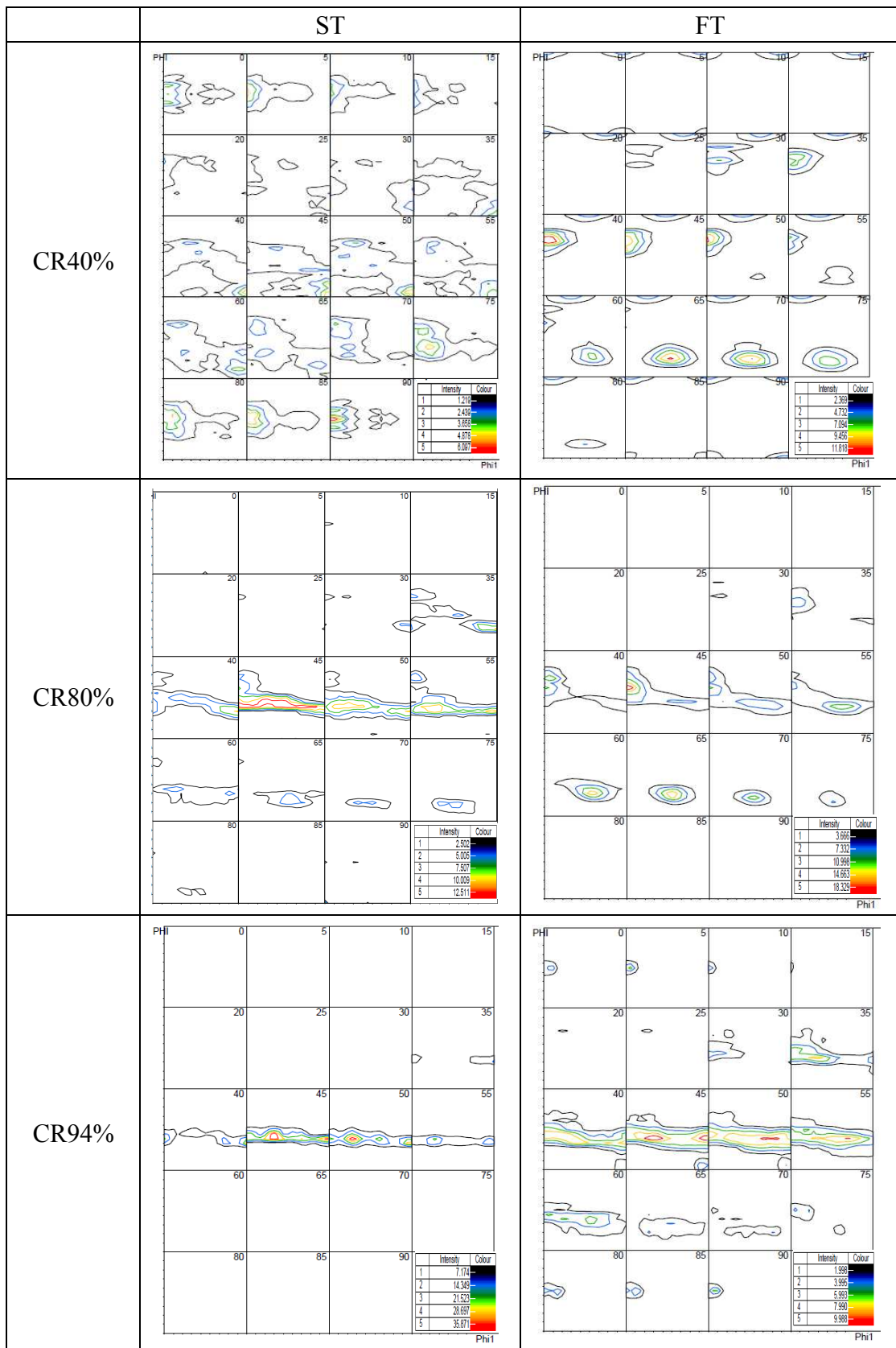
Fig. 6. Constant \phi_2 sections of ODF for Ti2448 alloy after different cold rolling rates followed by solution treatment (a, b, c) and flash thermal treatment (d, e, f).
