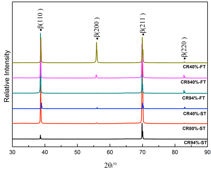
Fig. 1. XRD profiles of Ti2448 alloy after different thermo-mechanical treatments.
