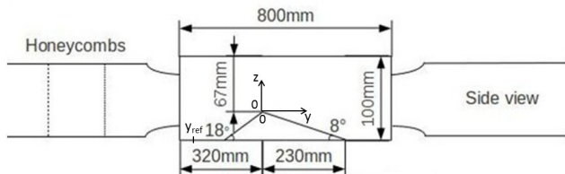
Figure 1: Test section of the experimental device using a Venturi profile ( H_{throat} = 67 mm is the reference length and y_{ref}^* = y_{ref}/H_{throat} = -3.7 ).
