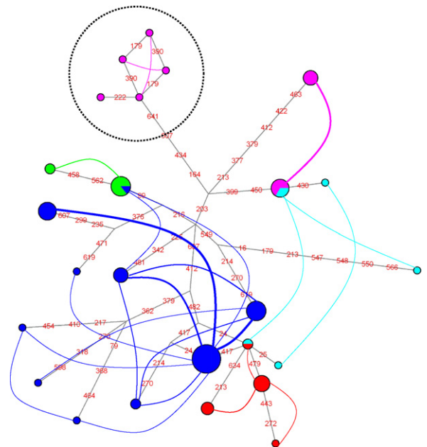
Fig. 4. Network of calmodulin haplotypes (dark blue: P. damicornis ; pink: P. meandrina ; green: P. ligulata ; pale blue: P. eydouxi ; red: P. molokenensis ).
