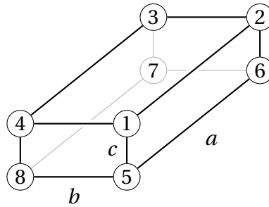
Figure 2: Rectangular parallelepiped.
