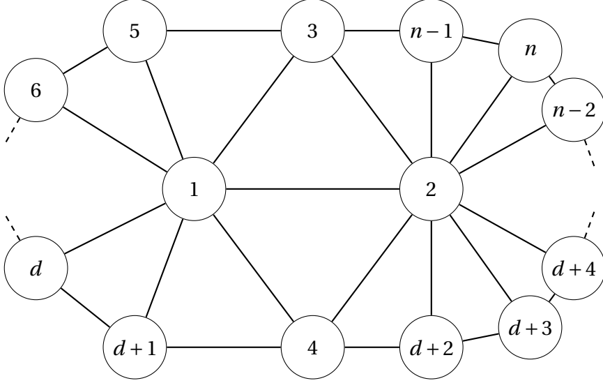
Figure 1: Generic description of \text{star}(1) \cup \text{star}(2) .
