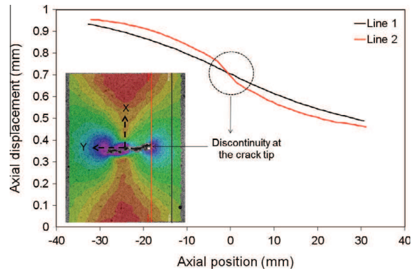
Fig. 10. Method for detecting the tip of transversal cracks associated with 0^\circ fibers failure.
