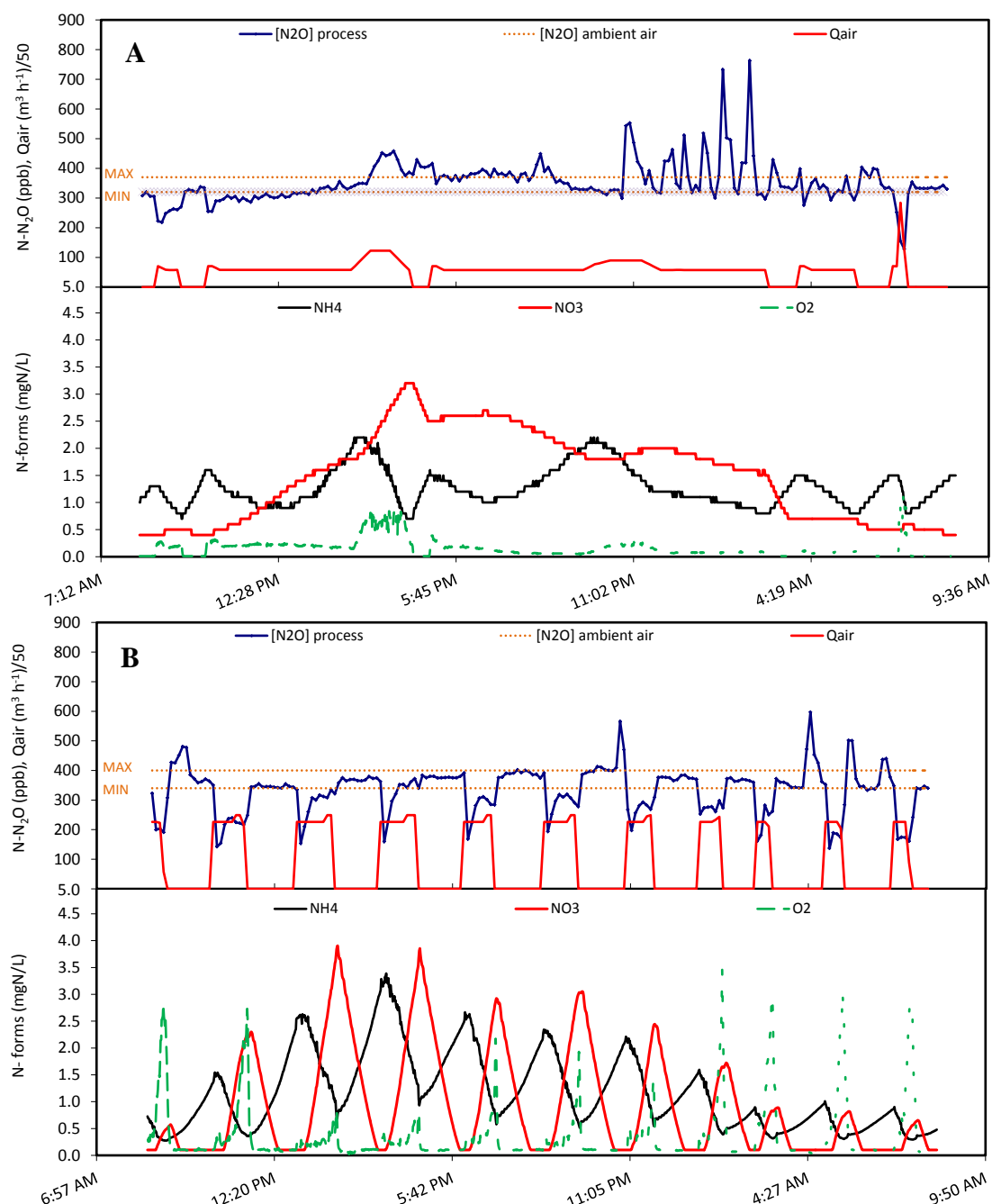
Figure 2. Off-gas N 2 O concentration, air flow and nitrogen forms concentration in tank 1 (A) and tank 2 (B) - aerated zones.
