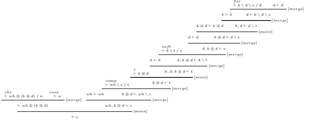
Figure 2: "che cosa \in fai ?" analyze
