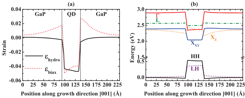
FIG. 2. (a) Hydrostatic ( \epsilon_{\text{hydro}} = \epsilon_{xx} + \epsilon_{yy} + \epsilon_{zz} ) and biaxial ( \epsilon_{\text{biax}} = 1/2(\epsilon_{xx} + \epsilon_{yy}) - \epsilon_{zz} ) strain components along the z [001] direction through the GaAs/GaP QD centre. (b) Confinement potentials along the z [001] direction through the QD centre calculated with the linear deformation potential theory using the hydrostatic and the biaxial strain components. Calculations are performed at 0 K.
