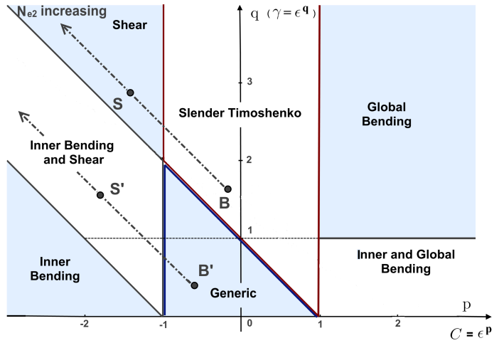
Figure 7. Behavior of the S_{structure} = N_{e_2} \times B_{eam} in relation to that of the primitive B_{eam} = N_{e_1} \times F_{frame} .
