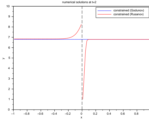
Fig. 4. Example of §4.5. Numerical solutions for 100 cells corresponding to the initial data (4.16) provided by the Godunov (blue) and Rusanov (red) schemes. In the case of the Rusanov scheme, numerical profiles are observed, as suggested by the study carried out in §3.2.
