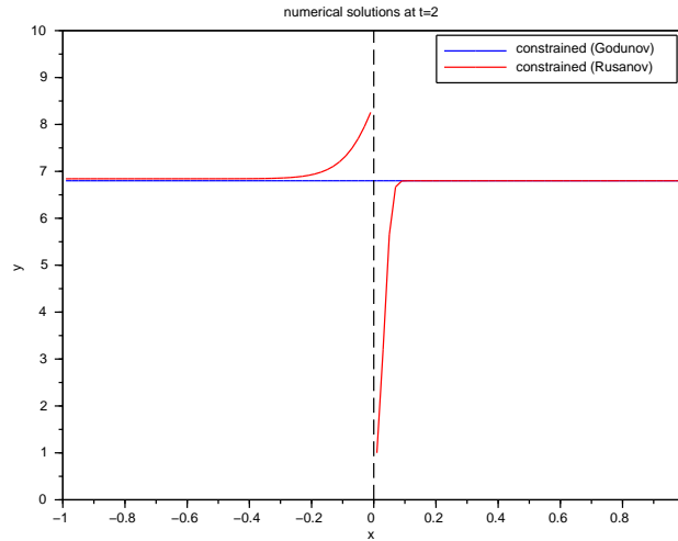
FIGURE 4. Numerical solutions for 100 cells corresponding to the initial data (83) provided by the Godunov (blue) and Rusanov (red) schemes. In the case of the Rusanov scheme, numerical profiles are observed, as suggested by the study carried out in §3.2.
