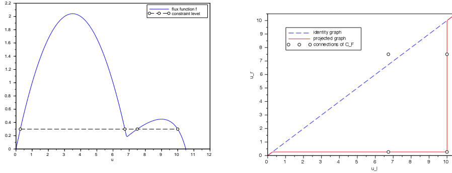
FIGURE 1. The flux function f , represented in the left figure, is not a bell-shaped function. Therefore, the set \mathfrak{C}_F contains 4 singletons represented in the right figure by black circles. The graph \beta (red solid line) is defined as the projection of the identity (blue dashed line) on the set of the maximal monotone graphs containing the strict connections of \mathfrak{C}_F located below the graph Id.
