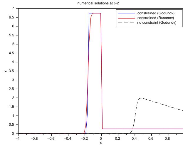
FIGURE 3. Despite the Rusanov scheme is more diffusive than the Godunov scheme, its numerical diffusion is well-balanced to preserve the connections of \mathcal{G}(\beta) (cf. Lemma 3.3), so that the undercompressive waves are accurately solved.
