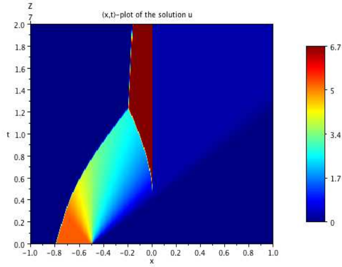
FIGURE 2. Plot of the solution u corresponding to the initial data (82) in the (x,t) -plane. One can see two waves leaving the interface, leading to a so-called undercompressive discontinuity, that is usually forbidden in the Kruzhkov theory
