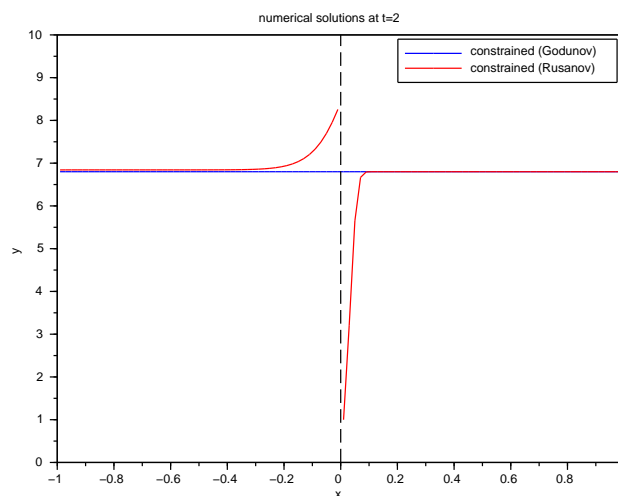
FIGURE 4. Numerical solutions for 100 cells corresponding to the initial data (83) provided by the Godunov (blue) and Rusanov (red) schemes. In the case of the Rusanov scheme, numerical profiles are observed, as suggested by the study carried out in §3.2.
