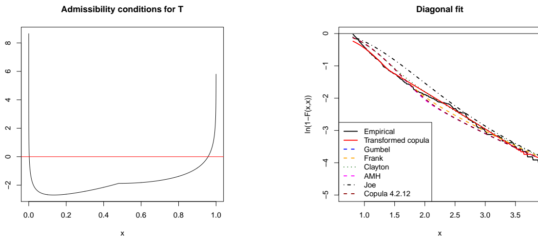
Figure 16: Left: Admissibility conditions in (28) for transformation T for the \mathcal{S}_1 with n = 500 . Right: Estimation of the 2-dimensional survival diagonal in logarithmic scale for \mathcal{S}_1 with n = 500 . Empirical diagonal is presented in black thick line; diagonal of the transformed model \tilde{F} in full red line; Gumbel model in blue dashed line; Frank model in orange dashed line; Clayton model in green dotted line; AMH model in violet dashed line; Joe model in black dashed-dotted line; Copula 4.2.12 in dashed dark red line.
