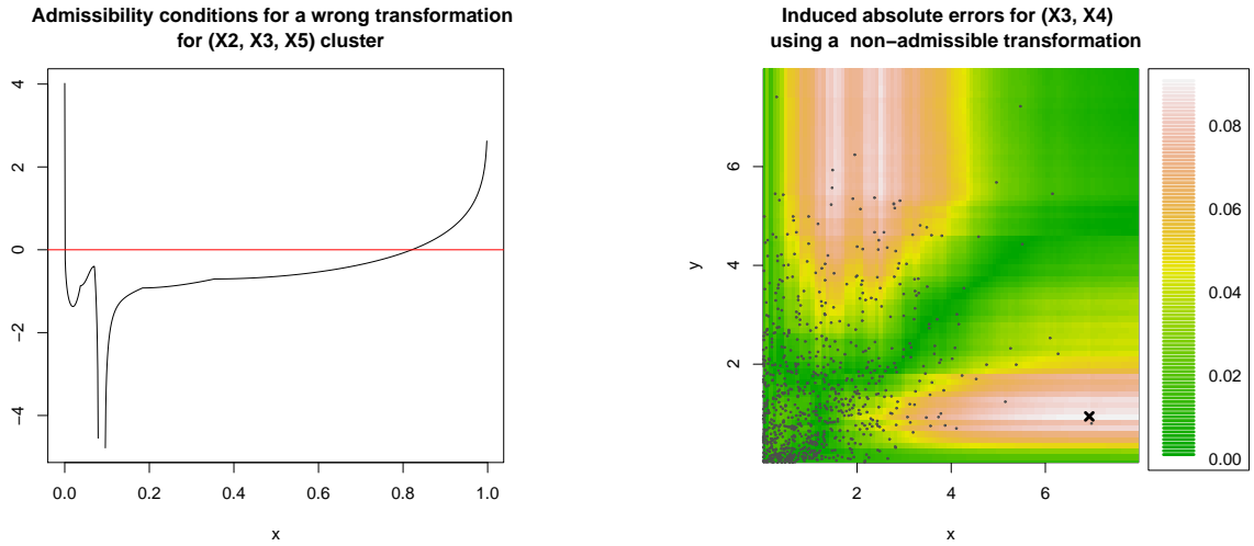
Figure 13: Left: Function m_\tau in (28) for a typical non-admissible external transformation \tau . This non-admissible transformation \tau corresponds here to a non-admissible external transformation T_A in (24) however leading to a good value of global MAE and SAE criteria for the final nested model in (26), \text{MAE} = 0.0057 and \text{SAE} = 0.0654 . Right: Errors |F_{(X_3, X_4)}(x, y) - F_n(x, y)| , for (x, y) in a lattice of 100 \times 100 points, where F_n is the empirical distribution function and F_{(X_3, X_4)} is the parametric nested model in (26) using the non-admissible external transformation \tau for the transformation T_A . Black cross represents the maximum error \text{SAE}_{3,4} = 0.0906 in the considered lattice. Black dots represent the associated rainfall data (X_3, X_4) .
