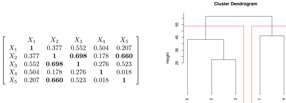
Figure 9: Left: Correlation matrix of the considered rainfall data. Correlations greater than 60% are indicated in bold font. Right: Dendrogram resulting to the hierarchical cluster analysis on the set of dissimilarities produced by the Euclidian distance on the rainfall data. Red boxes show the two considered clusters.
