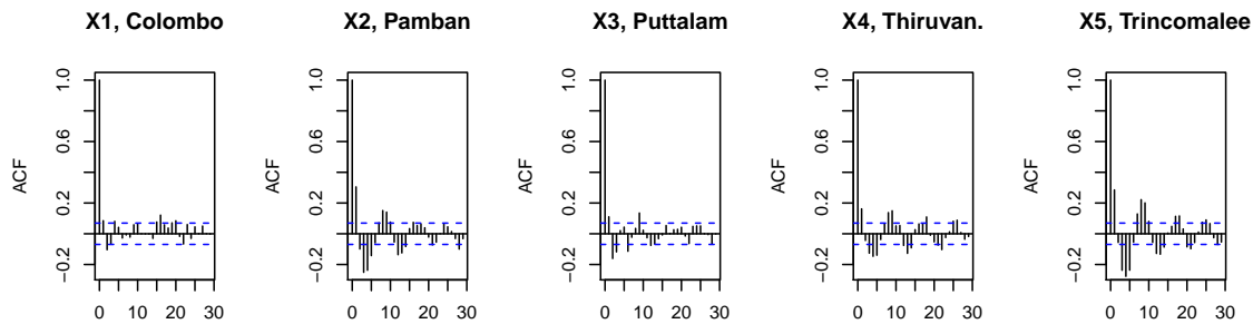
Figure 2: Estimates of the autocorrelation functions for the considered 5-dimensional rainfall data. Dotted horizontal lines give indicative 10% autocorrelation thresholds.
