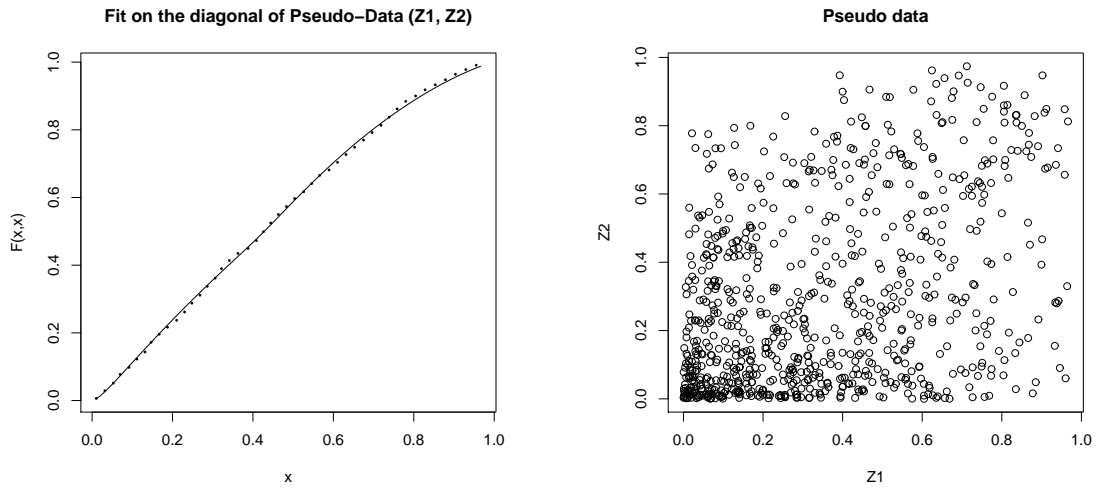
Figure 10: Left: Adjustment on the diagonal section for the pseudo-data (Z_1, Z_2) ; empirical estimation of the diagonal \hat{F}_{n, (Z_1, Z_2)}(x, x) (dotted line) versus our parametrical model (full line). Right: Plot of the pseudo-data (Z_1, Z_2) .
