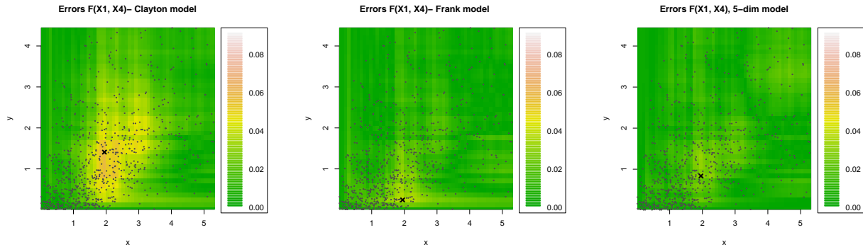
Figure 4: Errors |F_{(X_1, X_4)}(x, y) - F_n(x, y)| , for (x, y) in a lattice of 100 \times 100 points, where F_n is the empirical distribution function and F_{(X_1, X_4)} is parametric model with Gamma marginals and Clayton copula (left), Frank copula (centre panel). Errors of our transformed model \tilde{F} are displayed in the right plot. Black cross represents the maximum error SAE_{1,4} in the considered lattice (see (22)). Black dots represent the associated rainfall data (X_1, X_4) .
