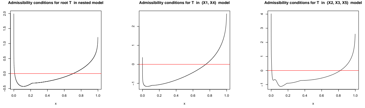
Figure 12: Admissibility conditions in (28) for transformations T in (26) (left) and T_B in (25) (centre panel) and T_A in (24) (right).
