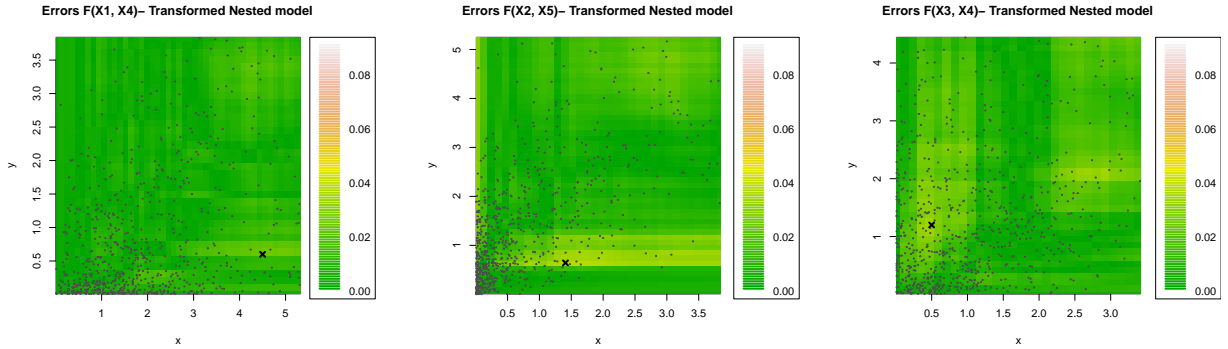
Figure 11: Errors |F_{(X_i, X_j)}(x, y) - F_n(x, y)| , for (x, y) in a lattice of 100 \times 100 points, where F_n is the empirical distribution function and F_{(X_i, X_j)} is the parametric nested model in (26) for (i, j) = (1, 4) (left), (i, j) = (2, 5) (centre panel), (i, j) = (3, 4) (right). Black cross represents the maximum error SAE_{i,j} in the considered lattice (see (22)). Black dots represent the associated rainfall data (X_i, X_j) .
