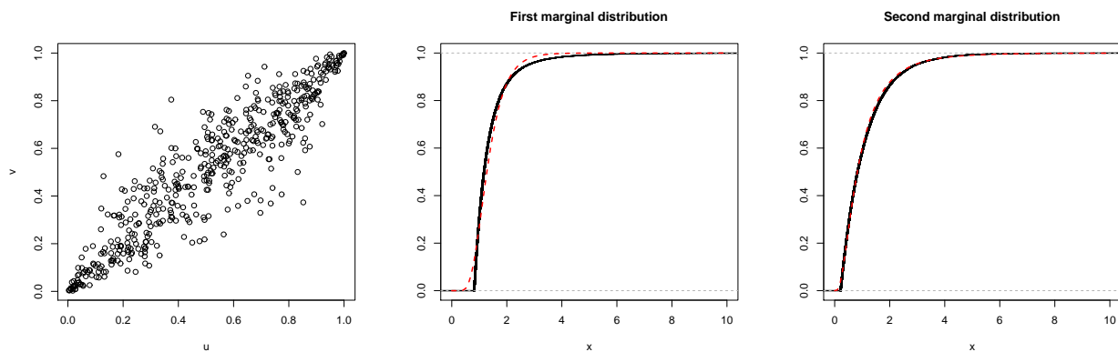
Figure 15: Pseudo-observations from the sample \mathcal{S}_1 with n = 500 from Copula 4.2.12 in Nelsen (1999) with \theta = 3 (left panel). The adjustment of marginals on the sample \mathcal{S}_1 is displayed in the centre and right panels using the log-normal distributions with parameters in Table 10 (dashed red lines). The marginal empirical distributions are represented using a black line.
