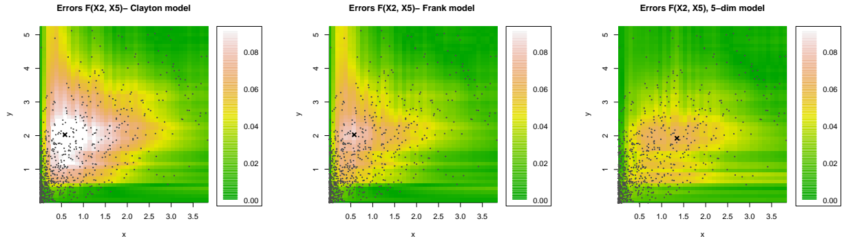
Figure 5: Errors |F_{(X_2, X_5)}(x, y) - F_n(x, y)| , for (x, y) in a lattice of 100 \times 100 points, where F_n is the empirical distribution function and F_{(X_2, X_5)} is parametric model with Gamma marginals and Clayton copula (left), Frank copula (centre panel). Errors of our transformed model \tilde{F} are displayed in the right plot. Black cross represents the maximum error SAE_{2,5} in the considered lattice (see (22)). Black dots represent the associated rainfall data (X_2, X_5) .
