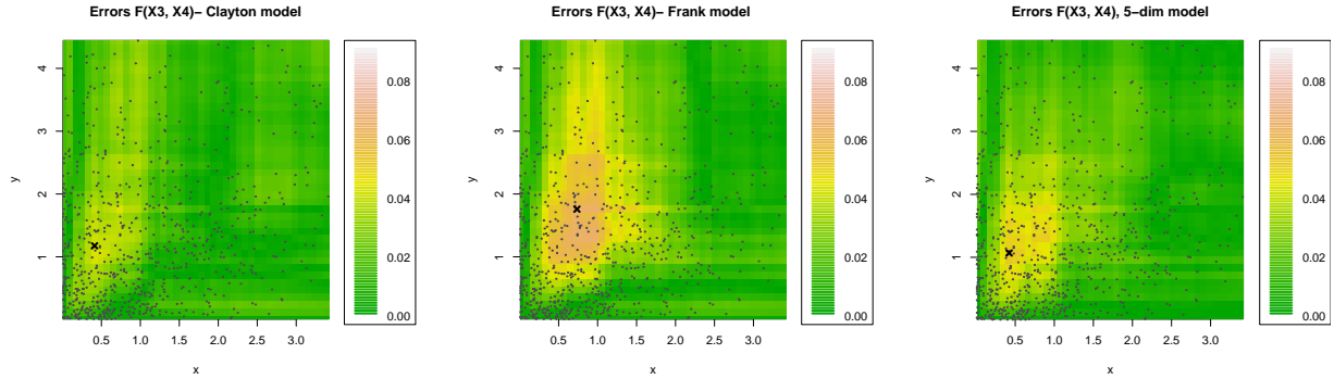
Figure 6: Errors |F_{(X_3, X_4)}(x, y) - F_n(x, y)| , for (x, y) in a lattice of 100 \times 100 points, where F_n is the empirical distribution function and F_{(X_3, X_4)} is parametric model with Gamma marginals and Clayton copula (left), Frank copula (centre panel). Errors of our transformed model \tilde{F} are displayed in the right plot. Black cross represents the maximum error SAE_{3,4} in the considered lattice (see (22)). Black dots represent the associated rainfall data (X_3, X_4) .
