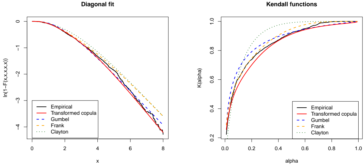
Figure 8: Left: Estimation of the 5-dimensional survival diagonal in logarithmic scale. Right: Kendall distribution function for the 5-dimensional rainfall data. Empirical diagonal and empirical Kendall (as in Barbe et al. (1996)) are presented in black thick line; diagonal of the transformed model \tilde{F} and associated K_{\tilde{\phi}} with \tilde{\phi} = \bar{T} \circ \exp(-t) in full red line; diagonal of parametric Gumbel model and K_{\phi_{Gumbel}} with \phi_{Gumbel}(t) = \exp(-t^{1/1.33}) in blue dashed line; diagonal of parametric Frank model and K_{\phi_{Frank}} with \phi_{Frank}(t) = -(\log(\exp(-x)(\exp(-2.45) - 1) + 1))/2.45 in orange thick dashed line; diagonal of parametric Clayton model and K_{\phi_{Clayton}} where \phi_{Clayton}(t) = (1 + t)^{-1/0.47} in green dotted line.
