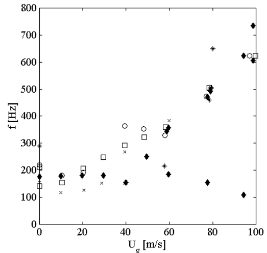
Figure 18: Variation of the frequency of the surface instability as a function of the gas velocity, for H_l = 0.7 mm and for all \alpha_{in} investigated: x \alpha_{in} = 0^\circ ; o \alpha_{in} = 30^\circ ; \square \alpha_{in} = 45^\circ ; \blacklozenge \alpha_{in} = 60^\circ ; * \alpha_{in} = 90^\circ .
