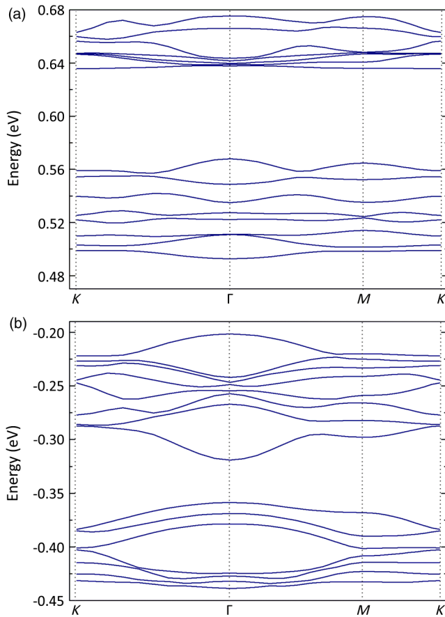
FIG. 9 (color online). (a) Lowest conduction bands and (b) highest valence bands of a graphene-type honeycomb lattice of truncated nanocubes of PbSe (body diagonal of 5.00 nm).
