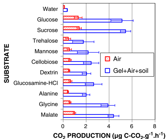
Fig. 10. Example illustrating microbial respiration rate for several added substrates. Microbial respiration rates have been estimated by taking into account either CO 2 accumulation in air only or CO 2 accumulation in the gel, air and soil solution minus the CO 2 issued from calcite dissolution.
