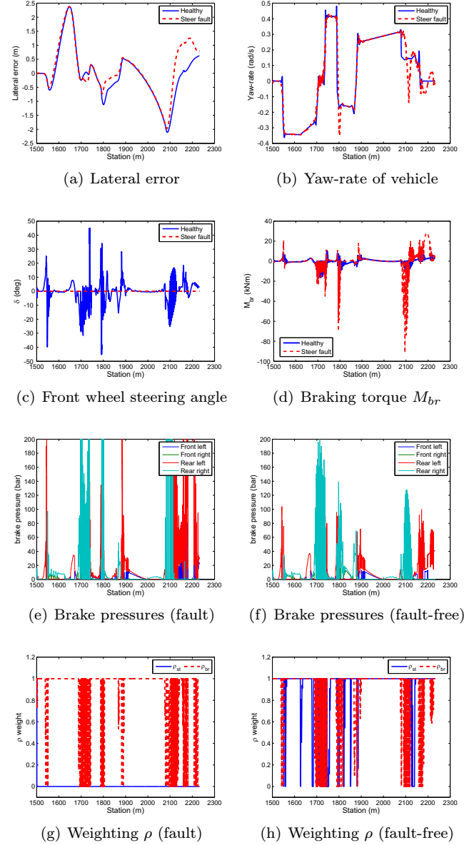
Fig. 8. Steering fault compared to the fault-free integrated control
