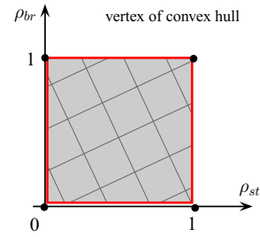
Fig. 6. Convex hull of LTI systems
