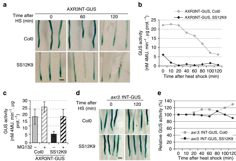
Figure 3 | ABP1 pathway stabilizes AUX/IAA repressors. (a) GUS staining in roots at various times after HS treatment of overnight ethanol-induced 4-day-old WT and SS12K9 seedlings expressing the pH5:AXR3NT-GUS construct. (b) Quantification and kinetic analyses of GUS activity in root samples as in a. Activity is expressed in 4-methylumbelliferone (MU) per minute and µg protein. (c) Quantification of GUS activity corresponding to accumulation of AXR3NT-GUS in overnight ethanol-induced roots treated or not with MG132 proteasome inhibitor during HS. Error bars represent s.d., n = 5 biological replicates. (d) GUS staining at various times after HS treatment in overnight ethanol-induced WT and SS12K9 roots expressing the pH5:axr3.1NT-GUS construct. (e) Quantification and kinetic analyses of GUS activity in root samples as in d. Scale bars, 500 µm (a,d).
