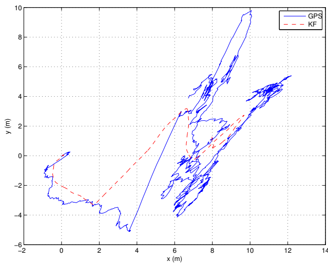
Fig. 9. GPS vs KF position.
