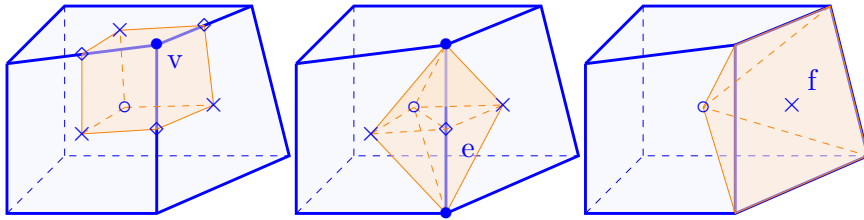
Figure 2: Hexahedral mesh cell c . Left: Example for \mathbf{p}_{\mathbf{v},c} ; Middle: Example for \mathbf{p}_{\mathbf{e},c} ; Right: Example for \mathbf{p}_{\mathbf{f},c} .
