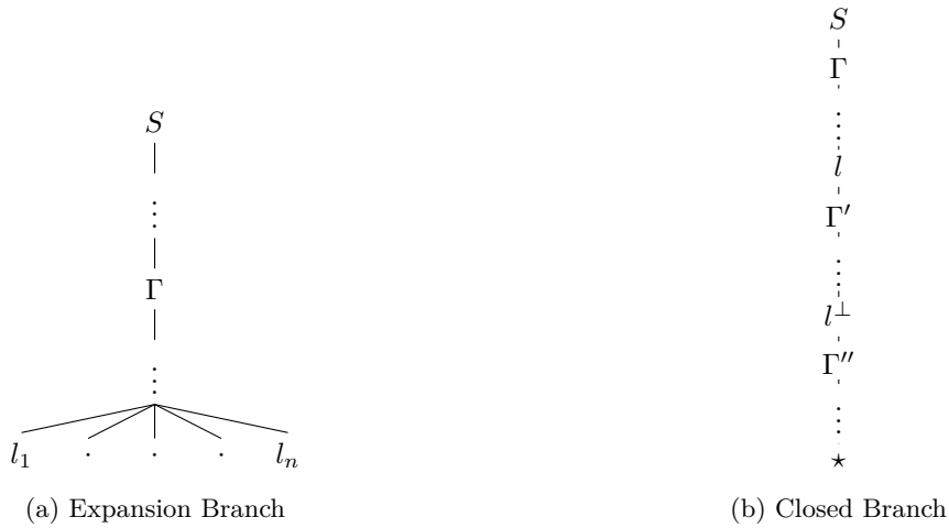
Figure 5.1: Clause Tableau
