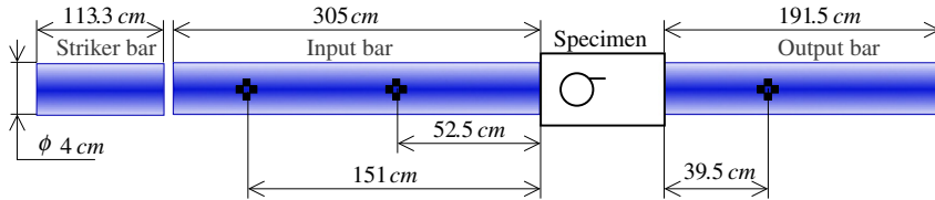
Fig. 1. Characteristics of the Split Hopkinson Pressure Bar.
