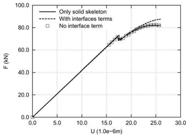
Fig. 10 Load-displacement curves
