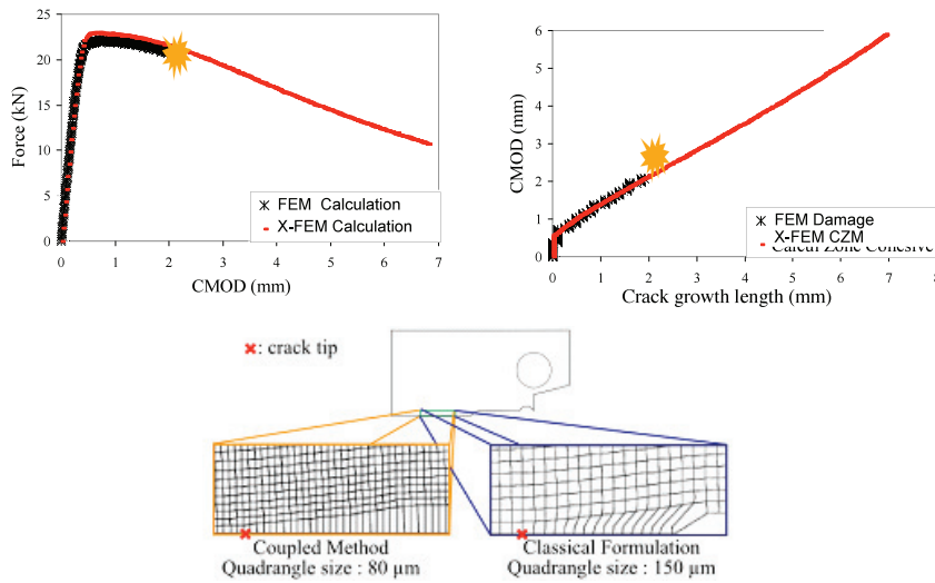
Fig. 10: comparison of Cohesive-XFEM predictions with standard damage modeling of crack propagation (CMOD= crack mouth opening displacements)
