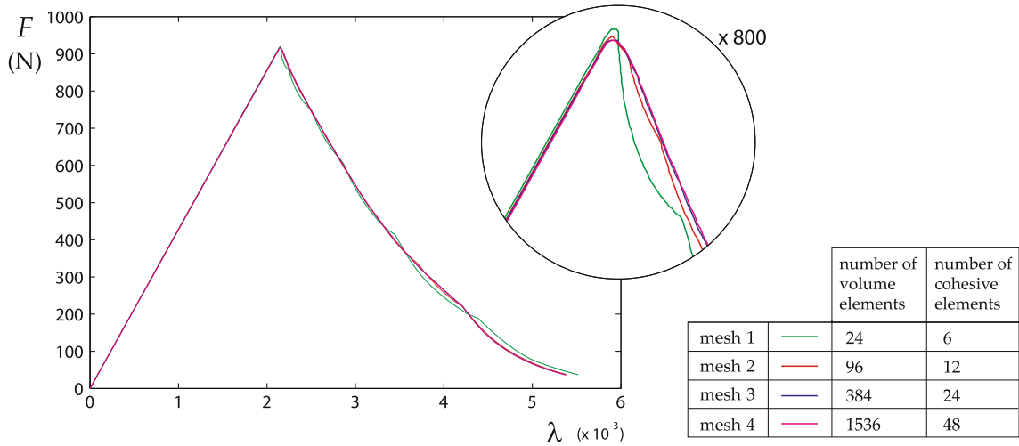
Fig. 10 Test example B: superposition of the loading curves obtained with all the meshes
