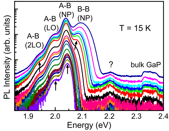
FIG. 3. Photoluminescence spectra from 3 nm MQW sample measured at 15 K as a function of excitation power ( 20 \mu\text{W} – 20 \text{ mW} ). The peaks due to NP acceptor-to-band [A-B(NP)], one LO phonon-assisted acceptor-to-band [A-B(LO)], two LO phonon-assisted acceptor-to-band [A-B(2LO)], and NP band-band [B-B(NP)] transitions are marked. The A-B transitions do not show blue-shift, whereas the B-B(NP) transition is strongly blue-shifted with increasing excitation power. The peak at \sim 2.2 \text{ eV} is not identified.
