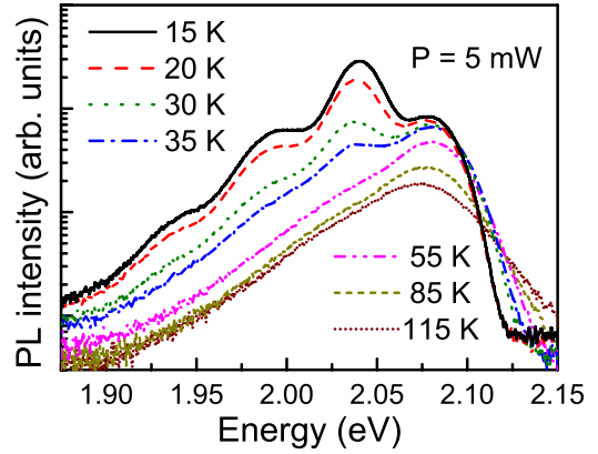
FIG. 5. Temperature dependence of the PL spectra for 3 nm MQW sample measured under 5 mW excitation power. Note that at higher temperature, band-to-band recombination dominates over the acceptor-to-band transitions.
