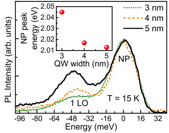
FIG. 2. Photoluminescence spectra from three AIP/GaP MQW samples measured at 15 K under very low excitation power ( \sim 20 \mu\text{W} ). The spectra have been scaled such that the prominent no-phonon (NP) peak in different samples has the same intensity and lies around zero energy. In each of the three cases, the lower intensity (phonon-assisted) peak is about 45–50 meV below the NP peak. Note that the intensity of the phonon peak relative to the NP peak increases with increasing well width. (Inset) The actual energy position of the NP peak as a function of the well width. The blue-shift in the NP peak energy with decreasing well width ascertains that the electrons are indeed those confined in the AIP QWs.
