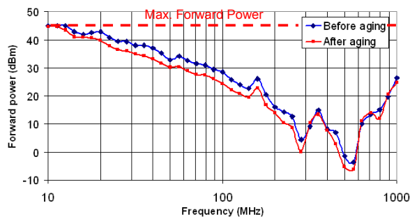
Figure 8. Evolution of the average susceptibility level of a PLL before and after an accelerated-life test [8]
