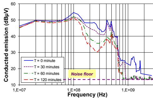
Figure 6. Evolution of the conducted emission of an I/O buffer after 120 minutes of 7 V electrical stress [5]
