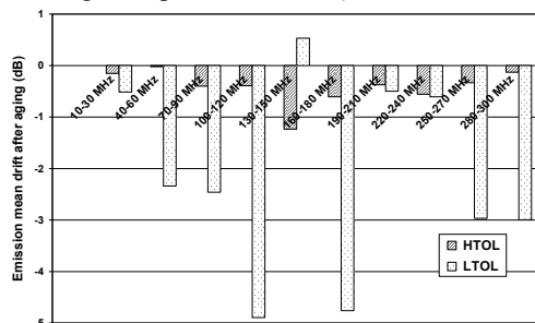
Figure 2. LTOL and HTOL aging impact on emission level (mean drift for all samples)
