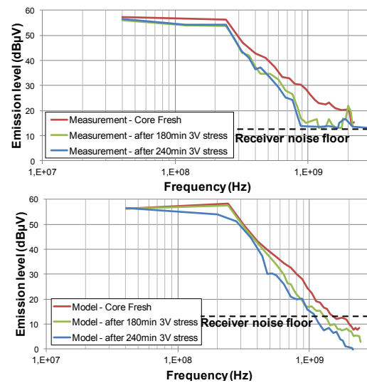
Figure 11. Measurement (top) and simulation (bottom) of the evolution of the conducted emission of a CMOS 90 nm digital core exposed to a 3 V electrical stress
