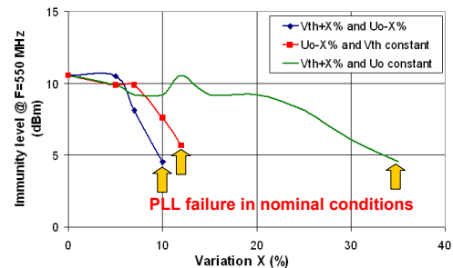
Figure 9. Simulation of the sensitivity of the PLL immunity level to variations of delay cell PMOSFET threshold voltage and mobility [8]
