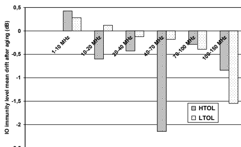
Figure 3. LTOL and HTOL aging impact on immunity level (mean drift for all samples)
