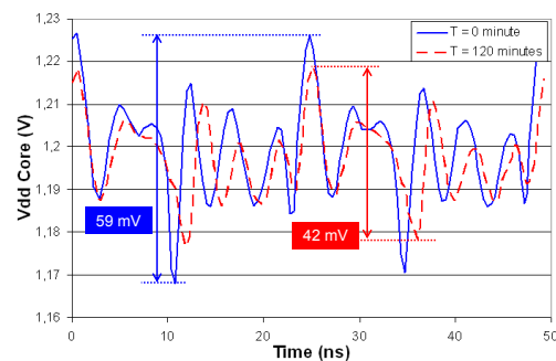
Figure 5. Evolution of the power supply voltage bounce of a digital core designed in CMOS 90 nm after 120 minutes of 3.6 V electrical stress [3]
