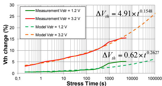
Figure 4. Measurement of V_{TH} evolution of 90 nm low voltage PMOS device exposed to negative gate-source voltage
