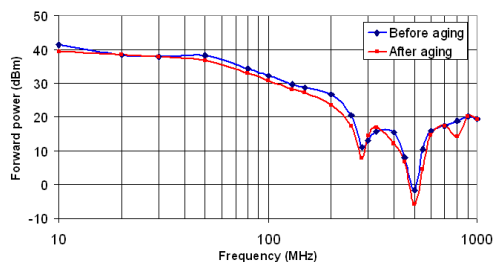
Figure 12. Simulation of the susceptibility level of the fresh and aged version of a CMOS 0.25 \mu\text{m} PLL [8]
