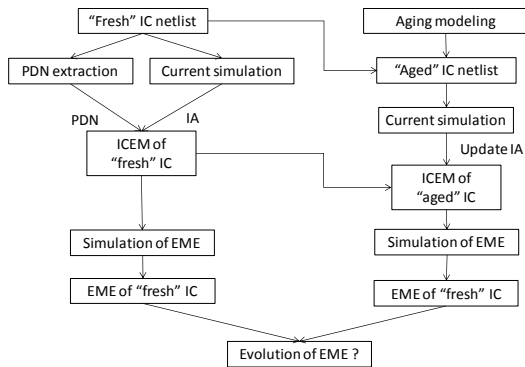
Figure 10. Aging-aware ICEM construction flow
