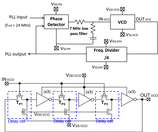
Figure 7. Internal structure of the tested PLL (top) and VCO (bottom) [8]
