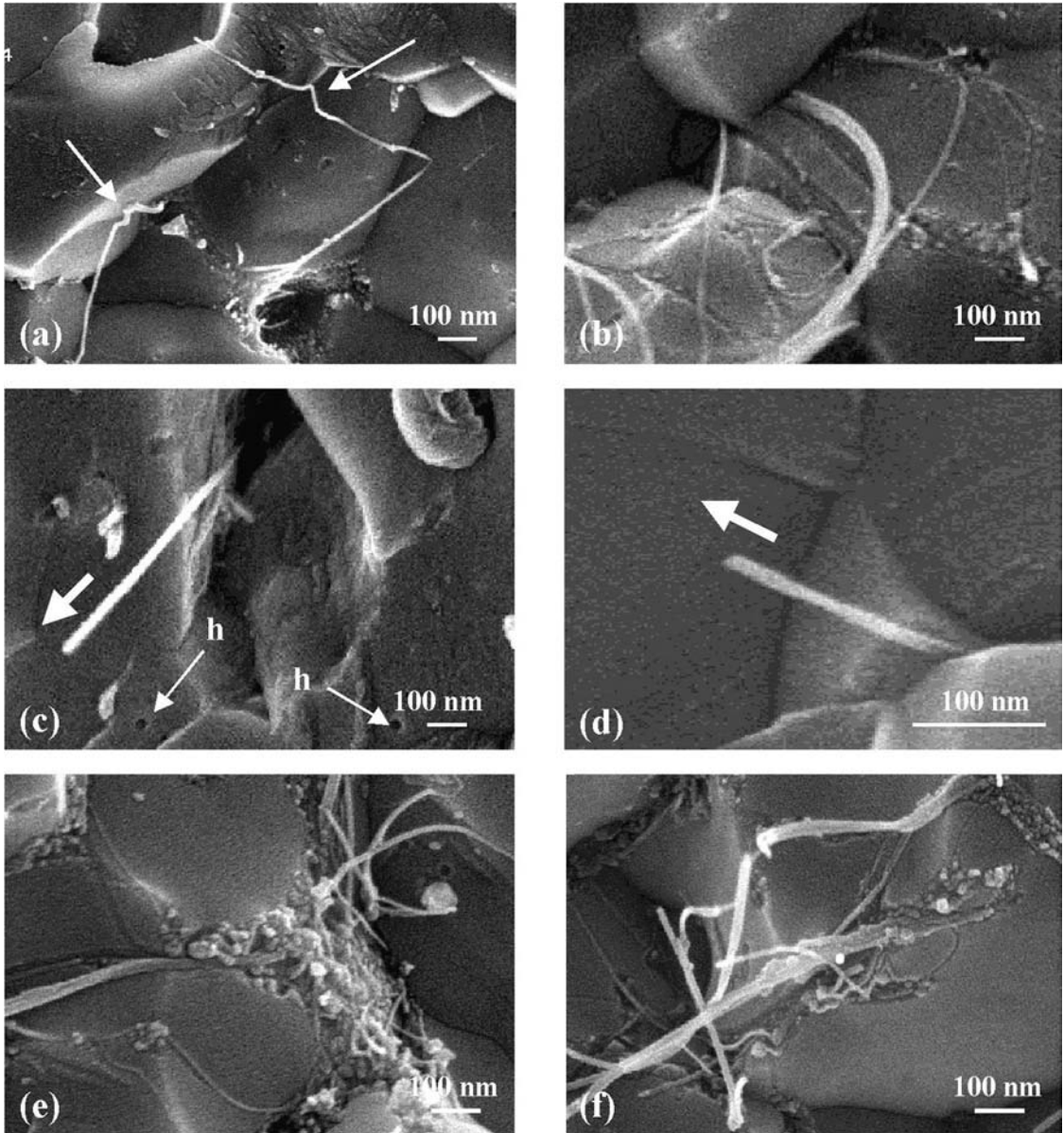
Fig. 3. SEM-FEG images of the fracture of the CNT-Fe- \text{Al}_2\text{O}_3 (CMA1) composite showing some aspects of the CNT-matrix interactions.
