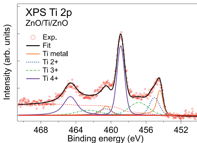
FIG. 3. Ti 2p spectrum of sample ZnO/Ti/ZnO recorded with 4 keV photon energy. The sample is highly oxidized. A weak metallic contribution is still present but the main Ti contribution corresponds to \text{Ti}^{4+} as in \text{TiO}_2 .
