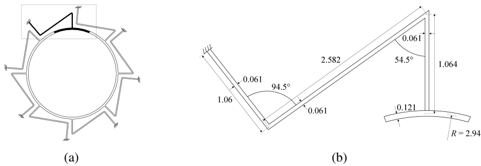
Figure 2. (a) Ring-based rate sensor with cyclic symmetry and its 45^\circ principal sector; (b) Actual modelled structure and its dimensions in mm (with axial thickness = 0.1 mm)
