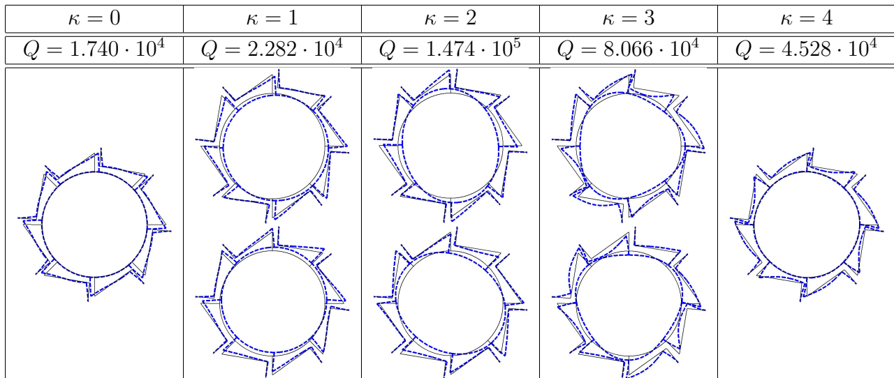
Figure 4. Mode shapes and calculated Q -factors of the ring-based rate sensor for the lowest natural frequency of each value of \kappa .
