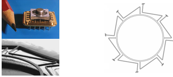
Figure 1. Photographs and schematic representation of the ring-based rate sensor and its leg shape
