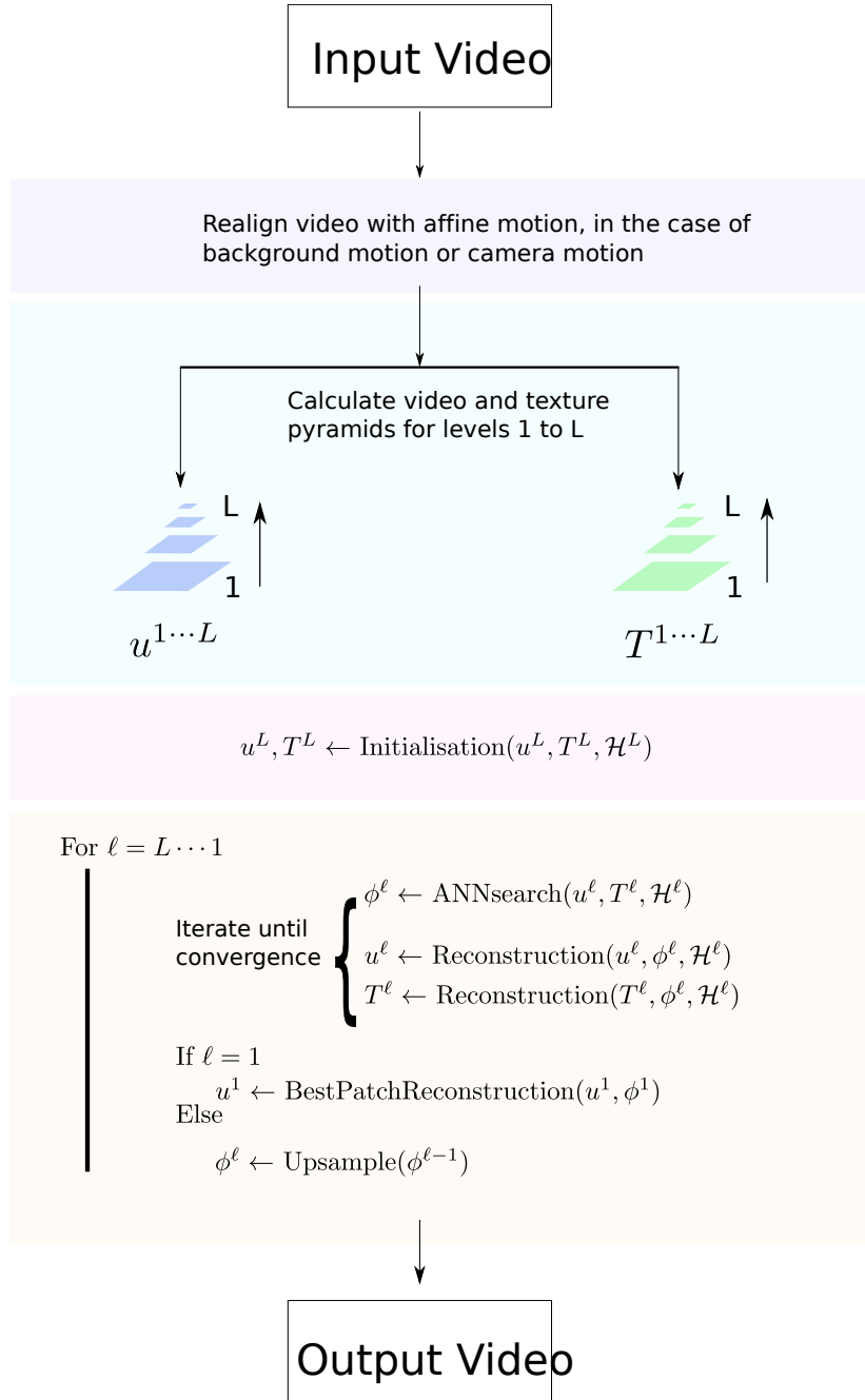
Figure 2. Diagram of the proposed video inpainting algorithm.
