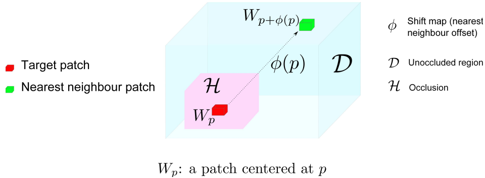
Figure 1. Illustration of the notation used for proposed video inpainting algorithm.
