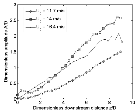
Figure 10: Dimensionless amplitude of the liquid jet as a function of dimensionless downstream distance to the injector for various U_g and U_l = 0.37 m/s.
