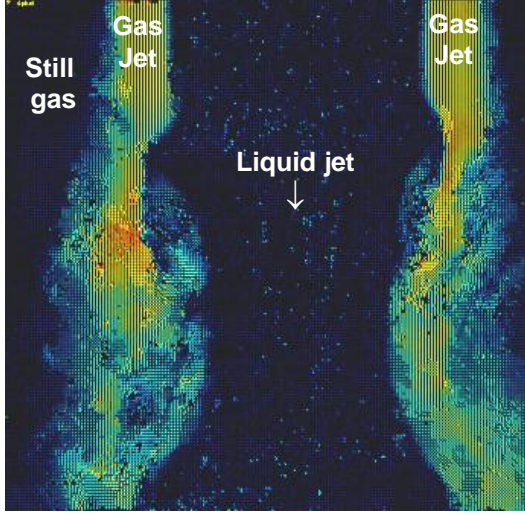
Figure 11: PIV visualization of gas flow around the liquid flow: non axi-symmetric KH wave induce non-axisymmetric recirculations.
