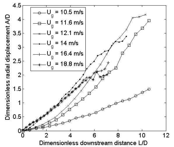
Figure 9: Dimensionless amplitude of the liquid jet as a function of dimensionless downstream distance to the injector for various U_g and U_l = 0.18 m/s.
