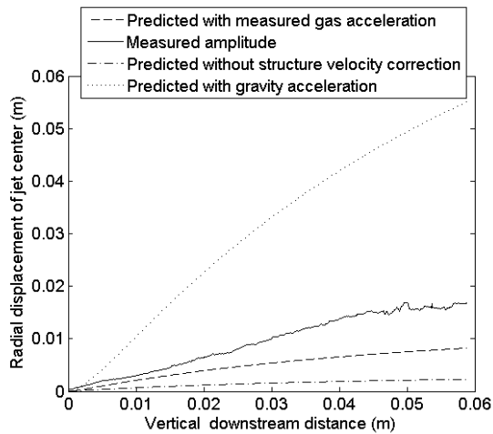
Figure 14: Predicted and measured radial displacement for U_g = 18.7 m/s and U_l = 0.18 m/s. Predictions with different hypotheses.
