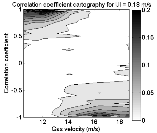
Figure 5: K-H wave mode dependency on gas velocity for a liquid velocity equal to 0.18 m/s.
