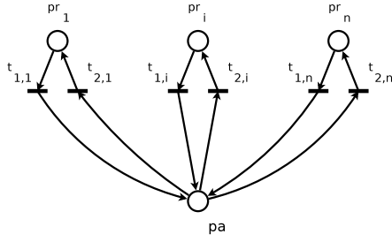
Fig. 9. Ability sub-net
