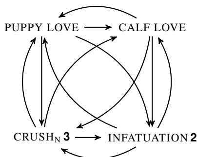
Figure 1: \text{Syn}_\cap saturated subgraph for synset (1)
