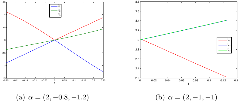
Figure 3: (\lambda_1(\Omega_t), \lambda_2(\Omega_t), \lambda_3(\Omega_t)) when \Omega_t is a parametrized ellipsoid of volume 4\pi/3
