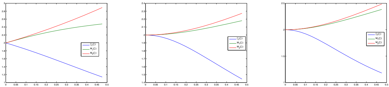
(a) Ellipses of area \pi , (b) 5 branches star-shaped domains \Omega_t (c) 7 branches star-shaped domains \Omega_t
