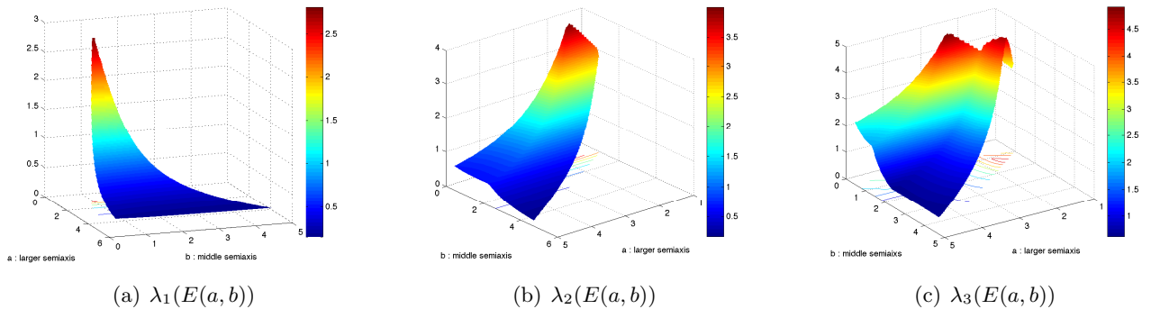
Figure 4: (\lambda_1(\Omega), \lambda_2(\Omega), \lambda_3(\Omega)) when \Omega = E(a, b) is an ellipsoid of volume 4\pi/3
