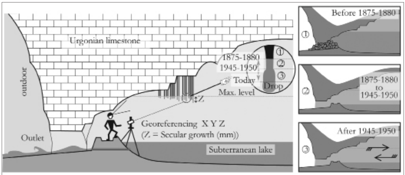
Figure 3: Location within the entrance chamber of the section of roof studied. The topography of the entrance room shows the proximity of the scarp. The three cross-sections show the general morphology of the room before entrance opening (upper), before ventilation by siphon lowering by cavers (2), and now (3).
