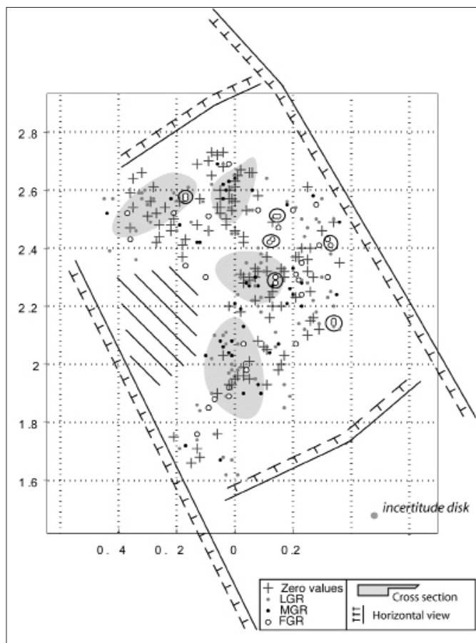
Fig. 6. Map of soda straw growth rates. The hatched area corresponds to an area without soda straws; the grey areas correspond to clusters of soda straws; the circles are the locations where FGR doublets are found. A small cross-section explains the reading of the barbed lines; the uncertainty disk shows the XY measurement uncertainty discussed in the text. Abscissa and ordinate units are meters.
