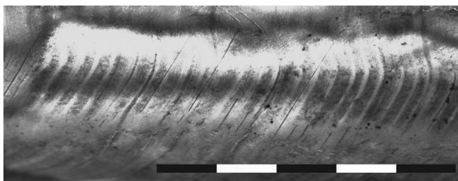
Zoom 1. U2.2-High growth rate lamination. The scale is five millimeters. Note the regularity of the annual lamination, which contrasts with the inter-annual thin laminae.
