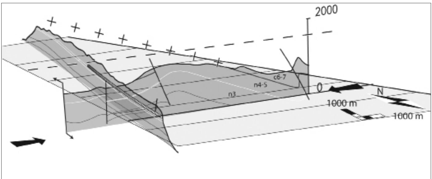
Fig. 2. Three-dimensional cross-section showing the location of cave passages.
