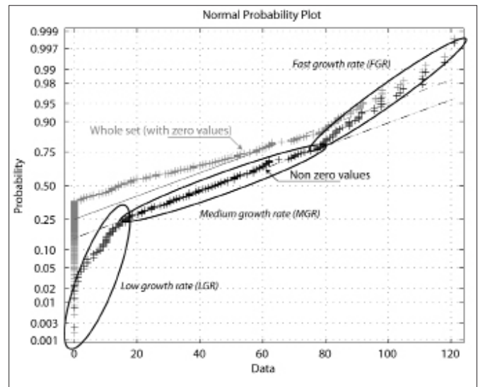
Fig. 4. Normal plot of the whole data set, with and without zero values. The abscissa shows the Z values (growth lengths) and the ordinate shows their occurrence probability in a Gaussian distribution. If the data represented a true Gaussian distribution, the graph would be a straight line. This is not the case for the whole data set, but three straight-line segments can clearly be distinguished for the non-zero values.
