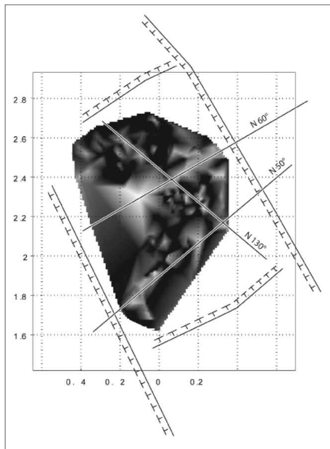
Fig. 7. Continuous mapping of soda straw growth rates. The rough lineation can be seen more clearly on this shades-of-grey map. The lighter greys correspond to the FGR and the darker greys correspond to the LGR. Abscissa and ordinate units are meters. The line corresponds to the bearings of the lineations.
