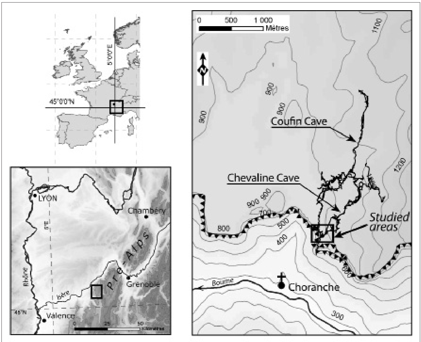
Fig. 1. Regional location map of the study area - the Choranche Caves in the Vercors Massif (France)
