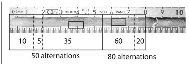
Photo 1. Soda straw from the entrance chamber, close to the study area (within a few meters). This soda straw is 8cm long. The most recent part is on the left. The tan-colored right-hand section is "dirty" calcite formed before the cave entrance was enlarged in 1875. The lamina counts are shown in the rectangles. The boxed sections of the soda straw are shown in close-up in Photo 2 (right-hand box) and Photo 3 (left-hand box).
