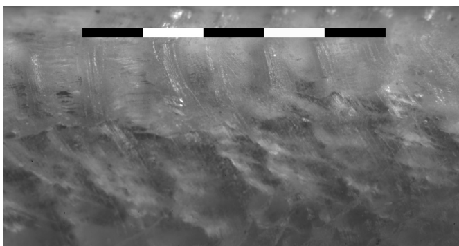
Zoom 2: U2.1 Low growth rate lamination.. The scale is five millimeters. Note the regularity of the annual lamination.
