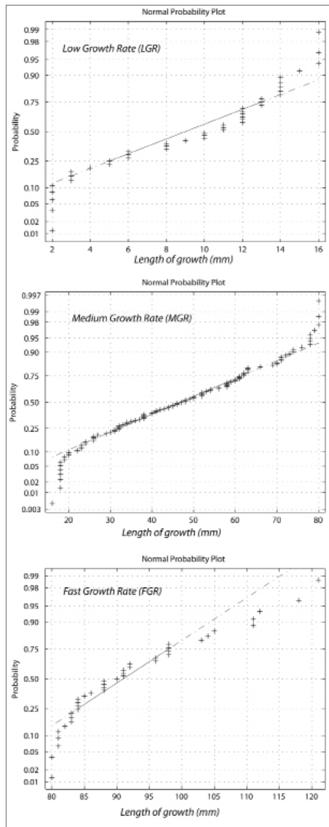
Fig. 5. Normal plots of the three growth rate subsets
