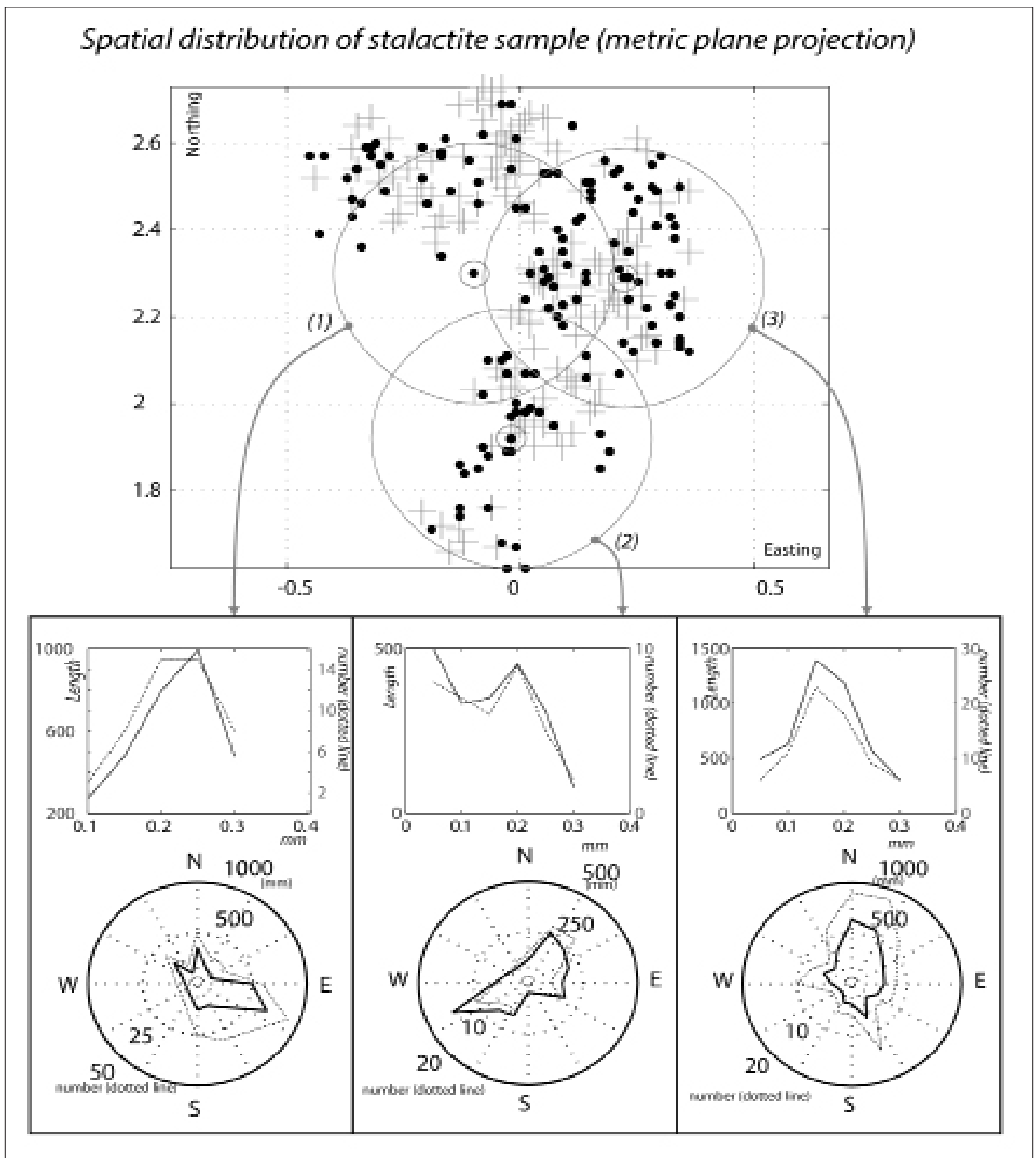
Fig. 8. Geostatistical results of the three fastest FGR. Two graphs are shown for each of the three fastest FGR (fastest of the three growth rates on the left, slowest on the right): a cumulative plot and a rose diagram. The upper graph shows the cumulative length and number (dotted line) of soda straws as a function of the distance from the FGR soda straw. Data are rough without correction of the area evolution.
