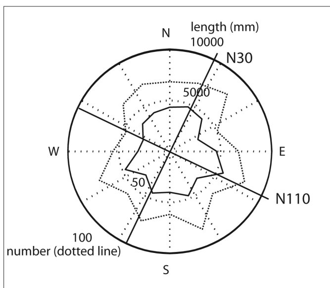
Fig. 9. Cumulative rose diagram. Rose diagram combining the plots for the 20 fastest FGR (see figure 10). No clear structure of these rose plots separately from the two slackened direction of N30 and N 110 which aren't statistically significant (ANOVA test).
