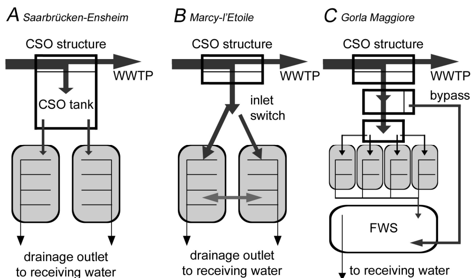
Figure 1. Simplified system sketch for in (A) retention soil filters in Germany; and (B) combined sewer overflow constructed wetlands in France; and (C) Italy.
