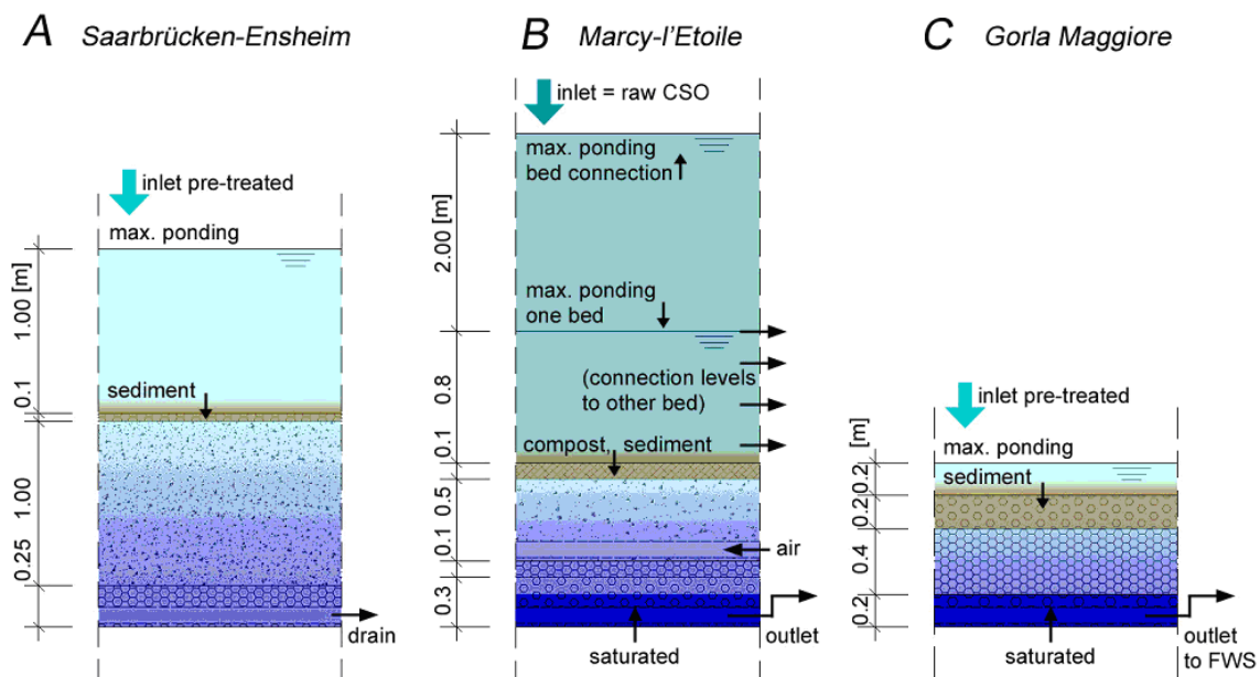
Figure 2. Simplified cross-sections of CSO-CWs in (A) Germany, (B) France; and (C) Italy.
