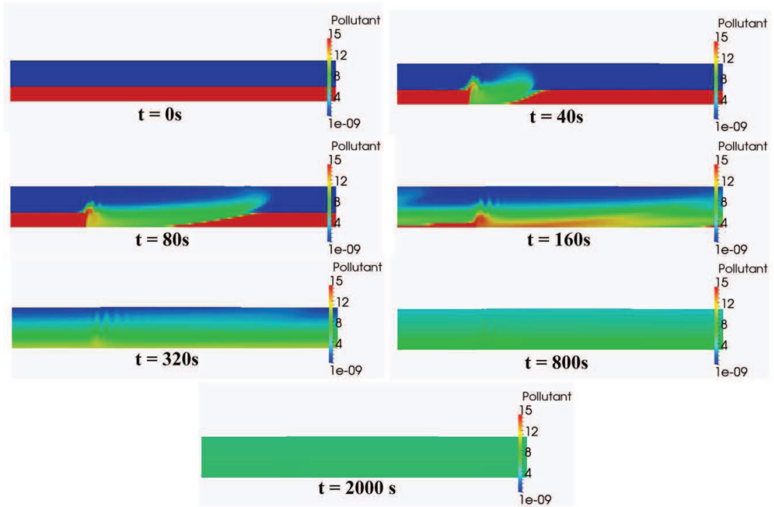
FIGURE 6. Snapshots of the tracer concentration in a raceway set into motion by a paddlwheel of angular velocity \omega = 0.85rad/s . It is clear that after several minutes, the raceway is totally homogeneous. Therefore, the paddlwheel has indeed the required effect on the mixing.
