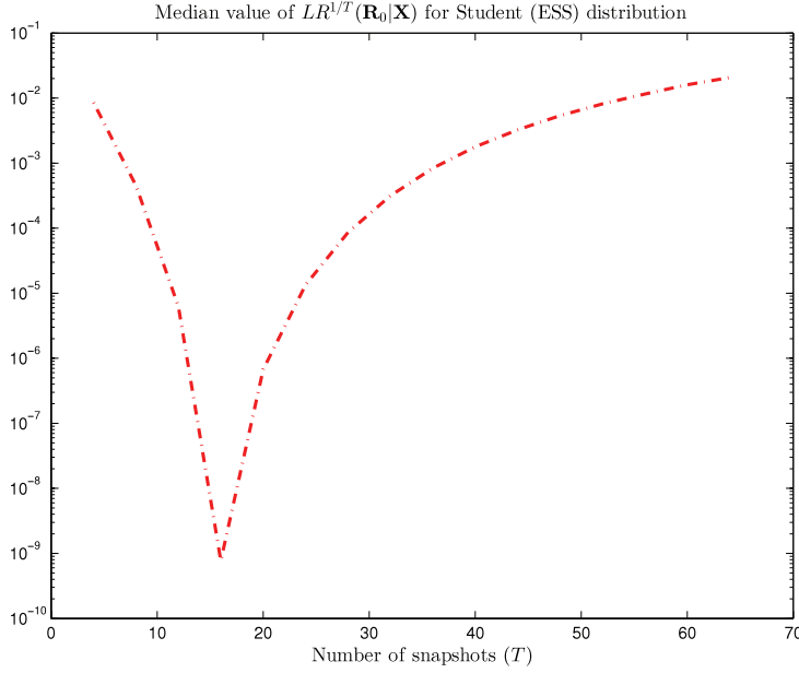
Fig. 2. Median value of LR^{1/T}(\mathbf{R}_0|\mathbf{X}) for a Student (ESS-type) distribution versus T . M = 16 and d = T .
